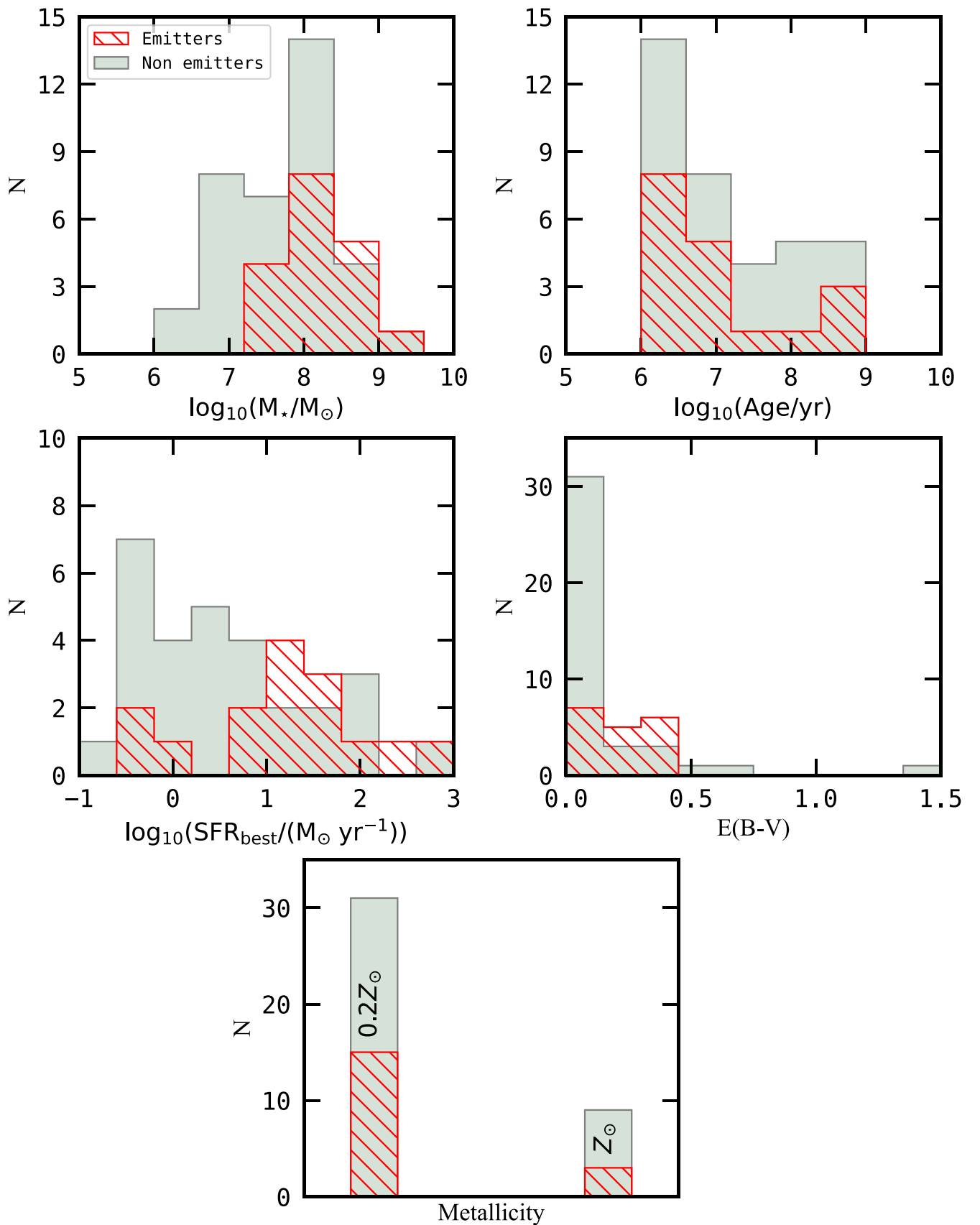
Figure 3. Comparison of the best-fit properties for emitters ( H\beta + [O\text{ III}] ) and H\alpha and nonemitters at z = 7-8 : stellar mass and age (upper row); star formation rate and color excess (middle row); and metallicity (bottom row). No significant differences have been noticed between the two populations for most of the stellar parameters, as determined by performing a two-sample Kolmogorov–Smirnov test. Differences in \text{SFR}_{\text{best}} between emitters and nonemitters might be explained by the fact that we are only looking at strong emitters that show a higher \text{SFR}_{\text{best}} .
