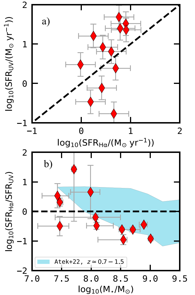
Figure 9. (a) Comparison between SFR _{\text{UV}} and SFR _{\text{H}\alpha} . The error bars reflect the usual scatter that has been observed with the Kennicutt’s relations we used to derive those two quantities. (b) The ratio of SFR _{\text{H}\alpha} and SFR _{\text{UV}} as a function of stellar mass. Both SFRs have been corrected by adopting the same reddening curve (Calzetti et al. 2000). The horizontal line indicates a one-to-one ratio. The pale blue shade refers to Atek et al. (2022) results at lower redshifts.
