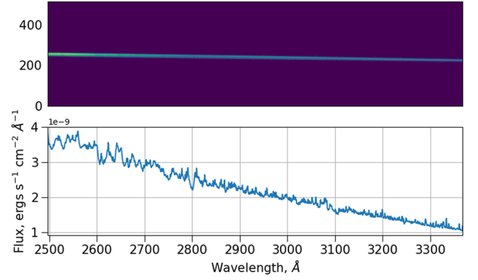
Figure 2. CUTE calibration observations of the O4 supergiant \zeta Puppis. The top plot shows the full-frame (2048 × 515 pixel) calibration image and the bottom plot shows the extracted one-dimensional spectrum (flux calibrated against archival HST and IUE spectra). \zeta Puppis was selected as a calibration target because of the wealth of archival NUV spectra and the high photospheric temperature ensures that iron and magnesium lines in the spectrum are narrow, interstellar features.
