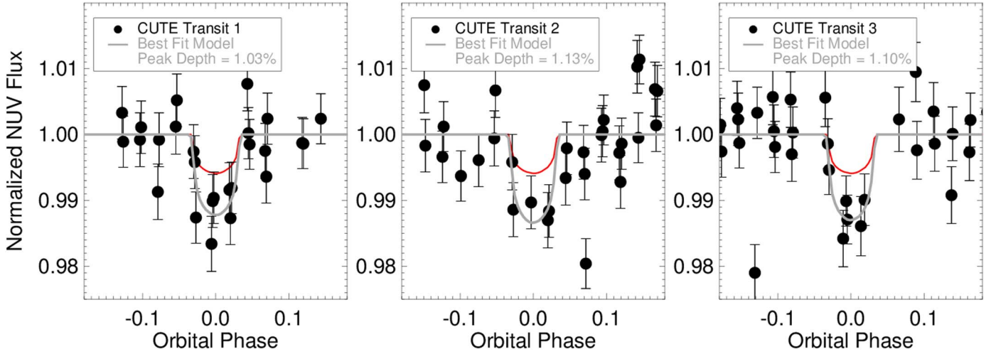
Figure 5. Initial CUTE light curves of WASP-189b, showing three independent NUV (approximately 2540–3300 Å) light curves (black points) and the best-fit transit models in gray. The plots compare the NUV band light curves with the optical light curve (in red) from CHEOPS (Lendl et al. 2020). The NUV transits are significantly deeper than their broadband optical counterparts, indicating an effective planetary radius increase of R_{p,NUV} \approx 1.5R_{p,opt} .
