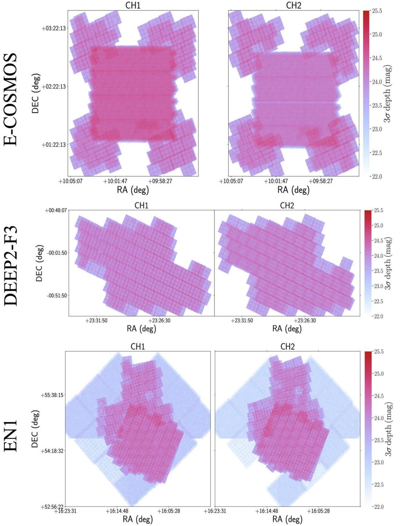
Figure 6. 3\sigma magnitude depths of the 3.6\ \mu\text{m} (left) and 4.5\ \mu\text{m} (right) mosaics. These are computed from Equation (1) based on the width of the distribution of fluxes measured in \sim 4000 empty apertures from the noise-normalized images (see text for details). We see that in the areas of interest (overlapping with the HSC-Deep layer) our mosaics have a 3\sigma depth of \sim 24 [AB] or better.
