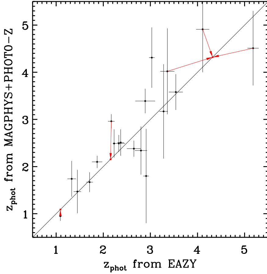
Figure A1. Comparison between z_{\text{phot}} from EAZY and MAGPHYS+PHOTOZ. Diagonal line shows equality for the two forms of z_{\text{phot}} . For three targets (UDS-ALMA 3, UDS-ALMA 5, EG-ALMA 6a/6b/6c) with known z_{\text{spec}} , red arrows connect the z_{\text{phot}} to the measured z_{\text{spec}} , indicated by red points.
