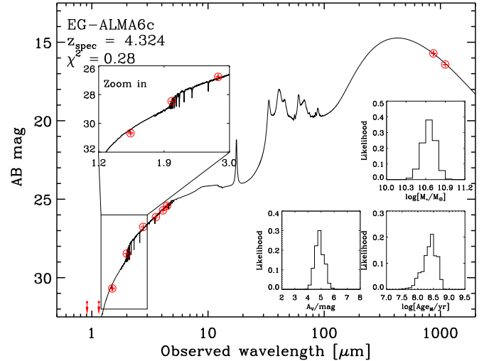
Figure C2. MAGPHYS fitting results for EG-ALMA 6 c. Red circles show the NIRCcam photometry (using a 0''.6 circular aperture) and the ALMA photometry. The two red arrows indicate the 3\sigma upper limits in the F090W and F115W bands. All values are demagnified. The black curve is the best-fitting model at the spectroscopic redshift z = 4.324 . The three insets on the right are the probability density functions of the stellar mass M_* , extinction A_V , and mass-weighted age. The inset on the left shows the SED near the Balmer break.
