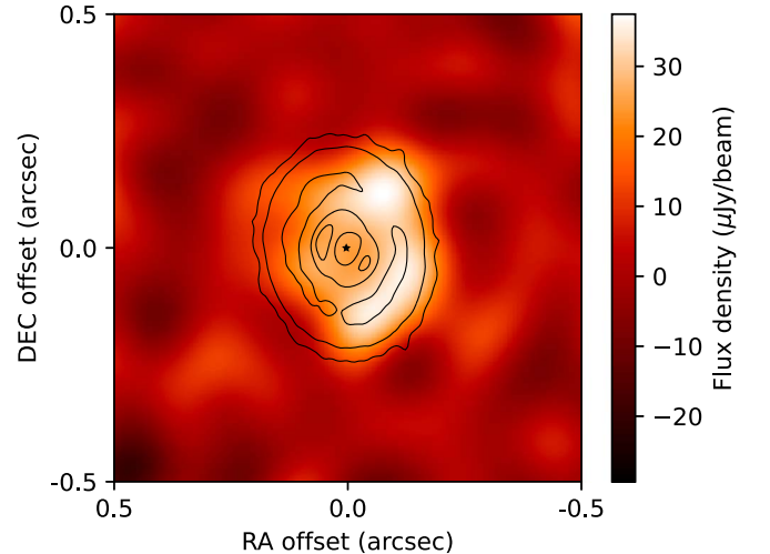
Figure 4. Zoomed-in Ka-band image ( 0''.18 \times 0''.16 ) superposed with contours of ALMA Band 7 image ( 54 \text{ mas} \times 37 \text{ mas} ; Pinilla et al. 2021). Contour levels are 17.1 \mu\text{Jy beam}^{-1} ( 1\sigma ) \times [5, 15, 45] . The stellar position is marked by a black star. VLA and ALMA FITS images shown in this figure are available as data behind the figure (see Figure 1).
