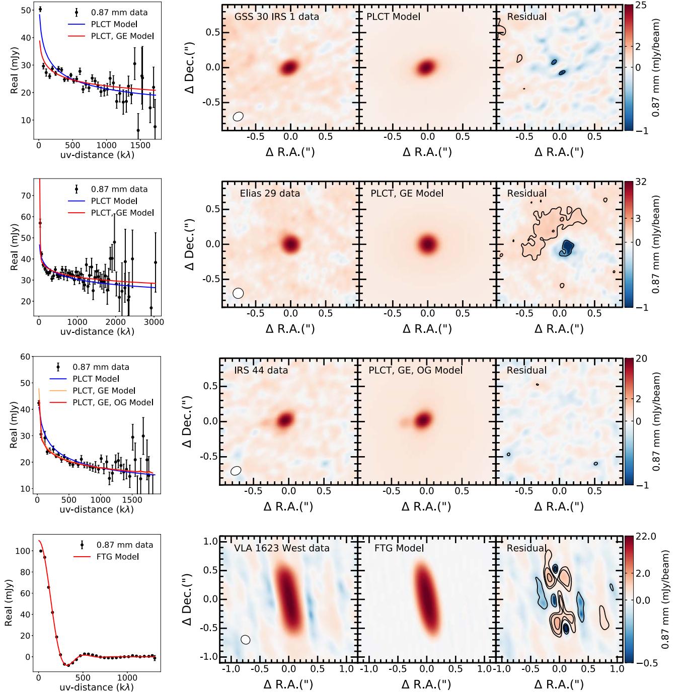
Figure 15. Same as Figure 3 for 0.87 mm data of the ambiguous disks. We show the UV data in 45 kλ bins.
