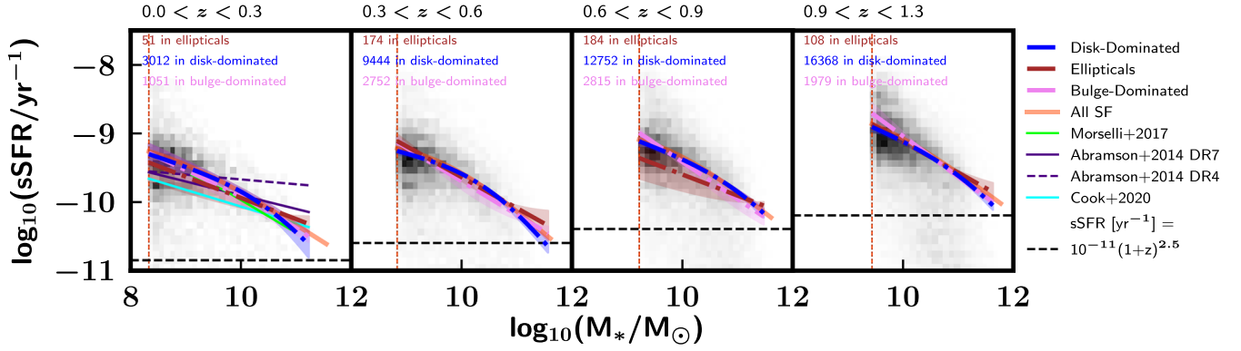
Figure 11. SFMS as estimated using only disk-dominated systems (BULG = 2 or 3, blue dashed–dotted), bulge-dominated disks (BULG = 0 or 1, magenta dashed–dotted), and elliptical systems (TYPE = 1, brown dashed–dotted) from the Zurich Structure & Morphology Catalog. Finally, we also include our global SFMS estimate in orange. We include the full sample as black density bins for reference. In the z < 0.3 subplot, we include literature from local studies such as the original Abramson et al. (2014) DR4 results showing a flat disk sSFR with mass (dashed violet) vs. the Abramson et al. (2014) DR7, Morselli et al. (2017), and Cook et al. (2020) results retaining a change in slope with stellar mass.
