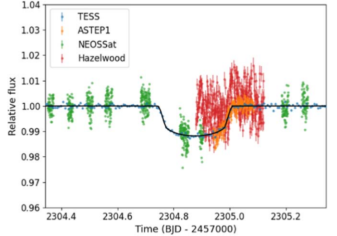
Figure 9. TESS FFI light curve for Sector 36 extracted with tesseract (blue points), ASTEP light curve (orange points), NEOSat light curve (green points), Hazelwood light curve (red points), and fitted model to the TESS data (black line) for transit 10.
