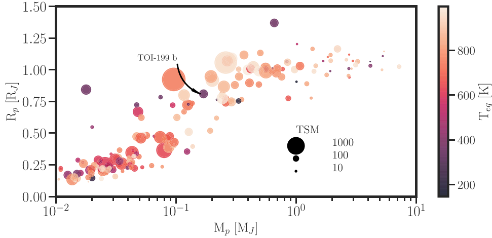
Figure 15. Mass–radius diagram for warm ( T_{\text{eq}} < 1000 \text{ K} ) giant planets with masses measured to better than 20% and radii measured to better than 10%, similar to our accuracies for TOI-199 b. The markers are color coded by equilibrium temperature and scaled by the TSM. TOI-199 b is significantly cooler than other well-characterized planets with similar masses and radii, and has a high TSM.
