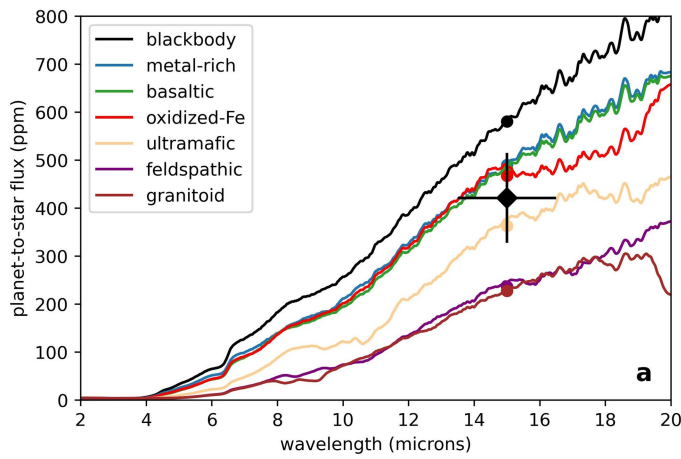
Extended Data Fig. 5 | Measured eclipse depth compared with a suite of simulated bare-rock emission spectra. a , Secondary eclipse spectra for various fresh surface compositions, assuming that TRAPPIST-1c is a bare rock. High-albedo feldspathic and granitoid surfaces are cool and fit the data moderately poorly ( 2\sigma ), as does a low-albedo and hot blackbody surface ( 1.7\sigma ). b , Space weathering by means of formation of iron nanoparticles (npFe) lowers
