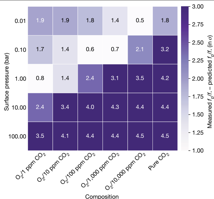
Fig. 2 | Grid plot comparing a suite of atmospheric models to the measured eclipse depth. Comparison between the measured eclipse depth and a suite of different \text{O}_2/\text{CO}_2 , cloud-free atmospheres for TRAPPIST-1 c with varying surface pressures and compositions. Darker grid cells indicate that we more strongly rule out this specific atmospheric scenario. The number in each cell is the difference between each model and the observations in units of \sigma . The lower the modelled atmosphere is in the grid, the higher its surface pressure. The rightmost column shows pure \text{CO}_2 atmospheres. The other columns are \text{O}_2 -dominated atmospheres with different amounts of \text{CO}_2 , ranging from 1 ppm ( =0.0001\% ) to 10,000 ppm ( =1\% ).
