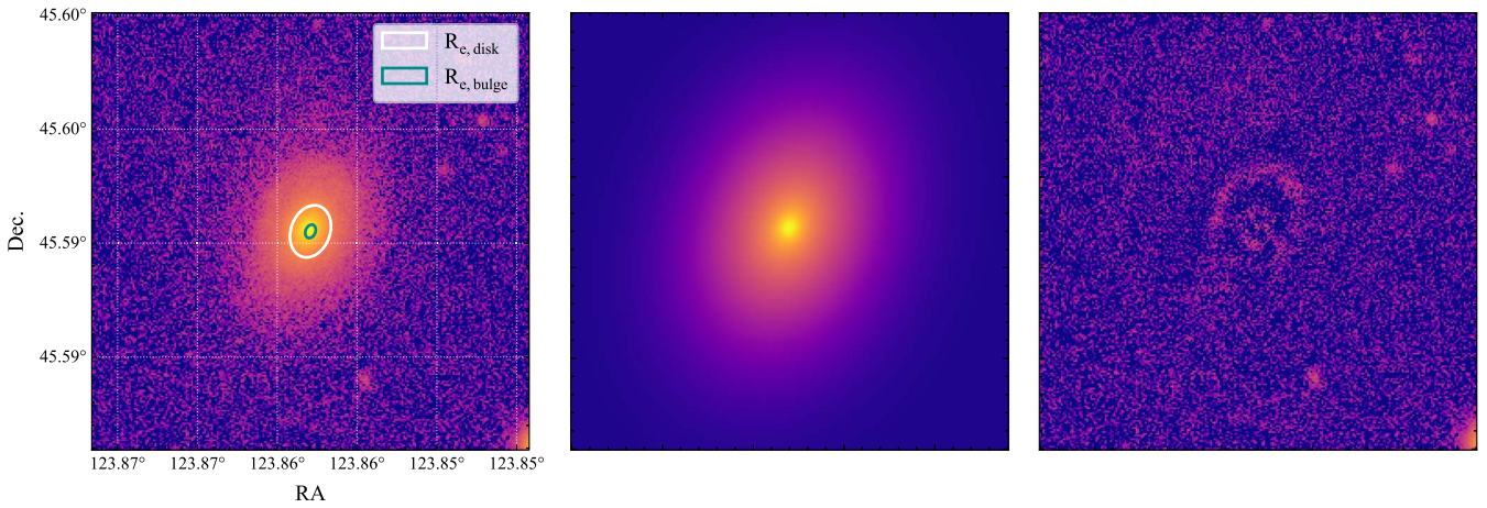
Figure 4. A 29'' \times 29'' cutout of the LMI observations of the host galaxy of AT2018bsi, shown with the GALFIT model and residuals. All images are on the same scale. GALFIT is able to model the host galaxy reasonably well with the residuals showing potential dust lane or spiral arm features, which are not as straightforward to model with GALFIT and for the purposes of the study presented here, are unimportant. In the left panel we show two ellipses representing the fitted bulge effective radius ( R_{e,bulge} , cyan) and the disk effective radius (where the relationship between the effective radius and the scale length of the disk is R_{e,disk} = 1.678R_{s,disk} , white).
