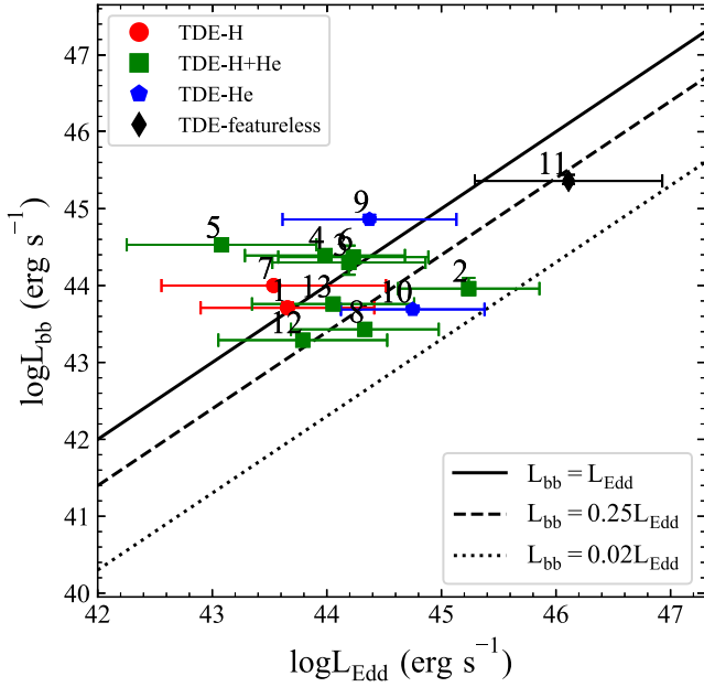
Figure 11. Peak blackbody luminosity as a function of the Eddington luminosity implied by the black hole mass. The solid, dashed, and dotted lines indicate constant Eddington ratios. We find that nearly all TDEs in our sample are consistent with being at or below the Eddington limit, with the exception of AT2018lna. This object has the lowest velocity dispersion in our sample and the black hole mass should be interpreted with caution. Labels for each TDE are in Table 1.
