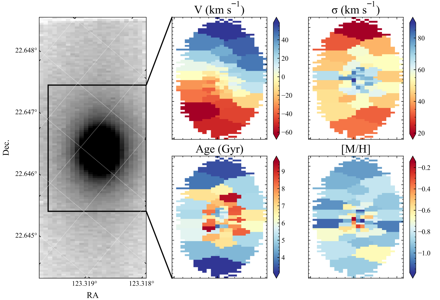
Figure 5. Example output from GIST of the host galaxy of AT2019azh. The left panel shows an unbinned white light image of the KCWI observation. The panels on the right depict the output maps from GIST, which show the ppxf -derived line-of-sight velocity, velocity dispersion, and stellar population ages and metallicities. The bins in this figure are constructed using the Voronoi binning method (Cappellari & Copin 2003) to reach a threshold S/N for each bin, in this case S/N \sim 10 . We note that Voronoi binning is not performed for the fits used in the analysis. This fit involves no spatial masking like that described in Section 2.2, but instead masks spaxels below the isophote level, which has a mean S/N of 2.2. This particular fit is not used for any analysis and is for illustrative purposes only.
