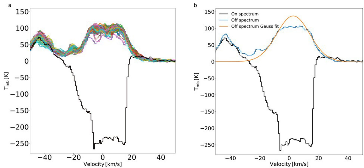
Extended Data Fig. 4 | HI spectra toward DR21. a, The HI absorption spectrum is shown in black, the 100 colored spectra represent the HI emission within a square of 20' \times 20' around DR21 in a grid of 1' . b, The black curve is again the absorption HI spectrum toward DR21, the blue curve is the HI emission spectrum (off), and the orange curve shows the Gaussian fit to the blue off spectrum.
