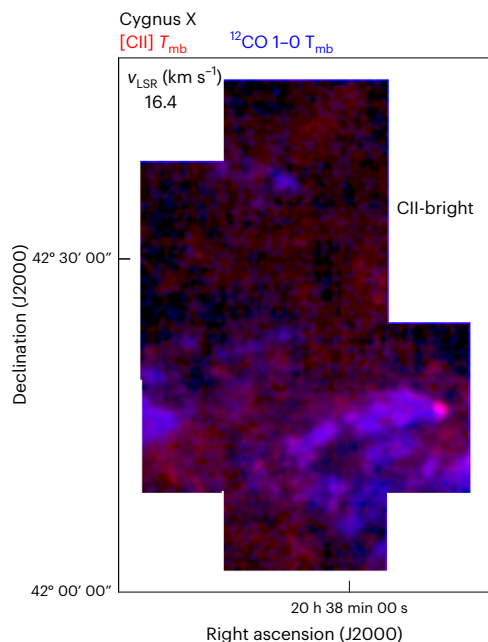
Fig. 2 | Video snapshot of [CII] and CO emission. The image displays a single velocity channel ( 16.4 \text{ km s}^{-1} ) of [CII] emission in red ( 0 to 16 \text{ K km s}^{-1} ) and CO emission in blue ( 0 to 25 \text{ K km s}^{-1} ), respectively, plotted as square-root values. Areas that are dark in CO (no or little emission) are bright in [CII] and reveal the large spatial extent of [CII] emission. The full video with all velocity channels can be found at https://astro.uni-koeln.de/stutzki/research/feedback/animations .
