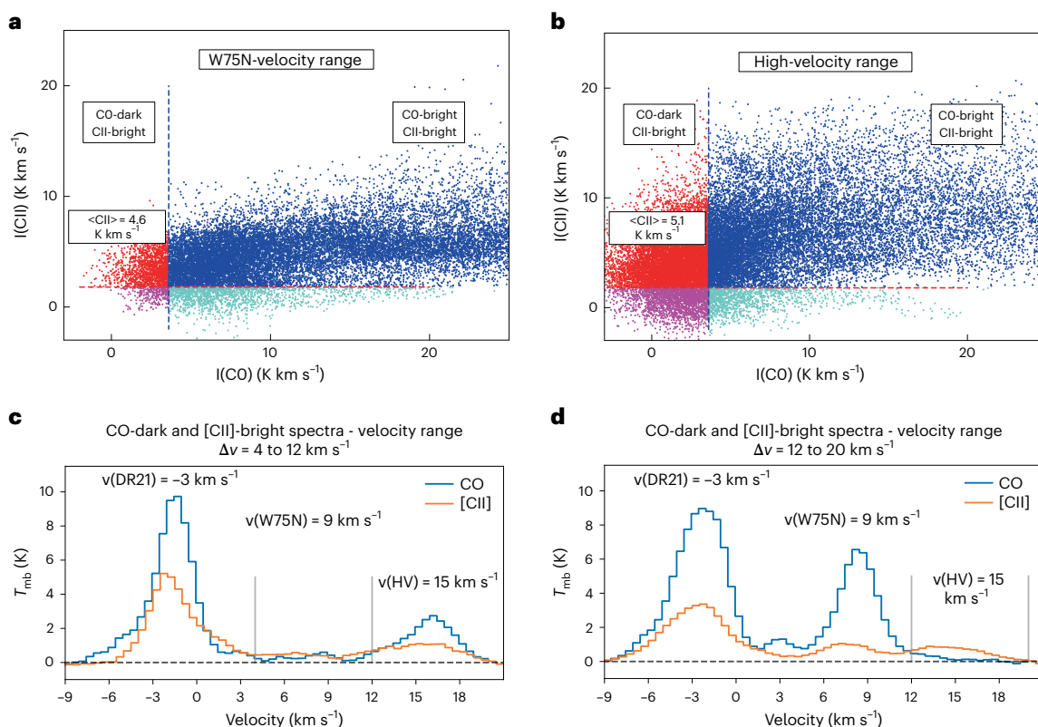
Fig. 3 | Scatter plots and spectra of [CII] and CO 1 \rightarrow 0 emission. a,b , The pixel-by-pixel correlations in the W75N ( a ) and HV ( b ) velocity ranges. The 3\sigma noise levels for [CII] emission ( 1.8 \text{ K km s}^{-1} ) and CO emission ( 3.6 \text{ K km s}^{-1} ) are indicated by red and blue dashed lines, respectively. The upper left area with red pixels indicates the intensity space that is below the CO noise level but bright in [CII], with an average value of 4.6 \text{ K km s}^{-1} (standard deviation 1.5 \text{ K km s}^{-1} ) and 5.1 \text{ K km s}^{-1} (standard deviation 2.2 \text{ K km s}^{-1} ) for the W75N and HV velocity ranges,
