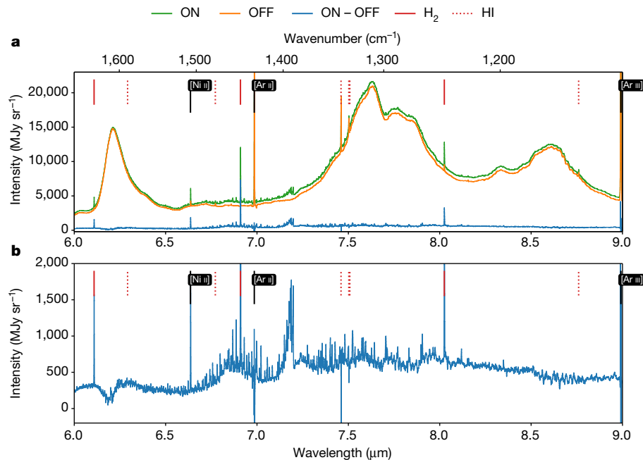
Fig. 2 | JWST-MIRI spectra of d203-506. a , Spectrum on the position of d203-506 (ON, green) and close to d203-506 (OFF, orange) over the 6–9 \mu\text{m} MIRI-MRS spectral range. The OFF spectrum is dominated by emission of the Orion Nebula:
