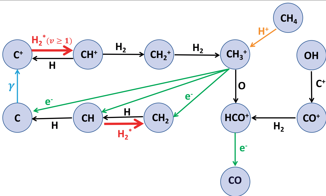
Extended Data Fig. 8 | Dominant \text{CH}_3^+ formation and destruction reactions at the \text{CH}_3^+ abundance peak predicted by the photochemical model shown in Fig. 7. This reaction network also leads to abundant \text{HCO}^+ in FUV-irradiated gas layers where x(\text{C}^+) > x(\text{CO}) . Red arrows show endoergic reactions when \text{H}_2 is
