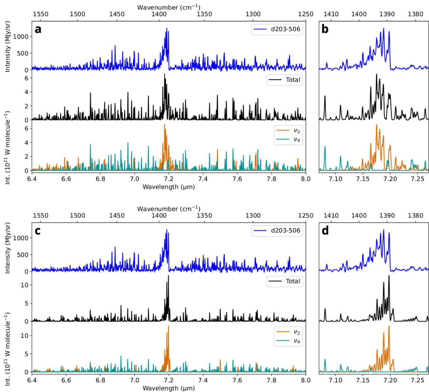
Extended Data Fig. 4 | Spectroscopic models I and II. a , Model I, with zoom on the strongest lines ( b ). c , Model II, with zoom on the strongest lines ( d ). For these models, the excitation temperature is T=400 K, and we use a Gaussian profile of 0.35\text{ cm}^{-1} full-width-at-half-maximum.
