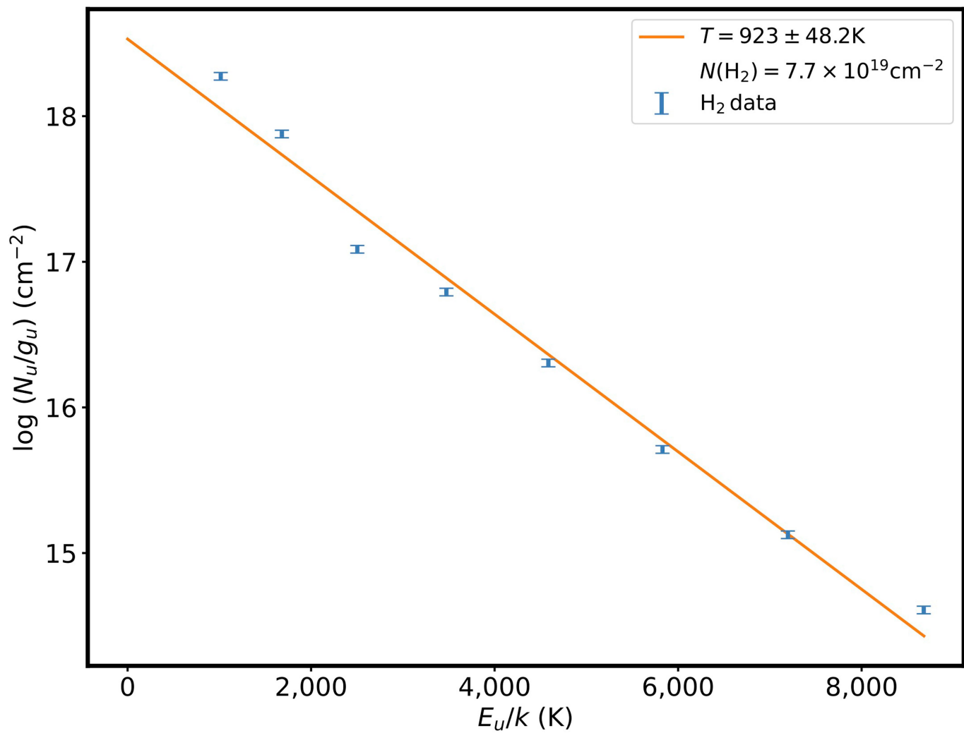
Extended Data Fig. 3 | H 2 excitation diagram derived from the line intensities in Extended Data Table 2 using the H 2 toolbox (see Methods for details). Error bars result from the propagation of the absolute calibration error of MIRI, which we take from ref. 58.
