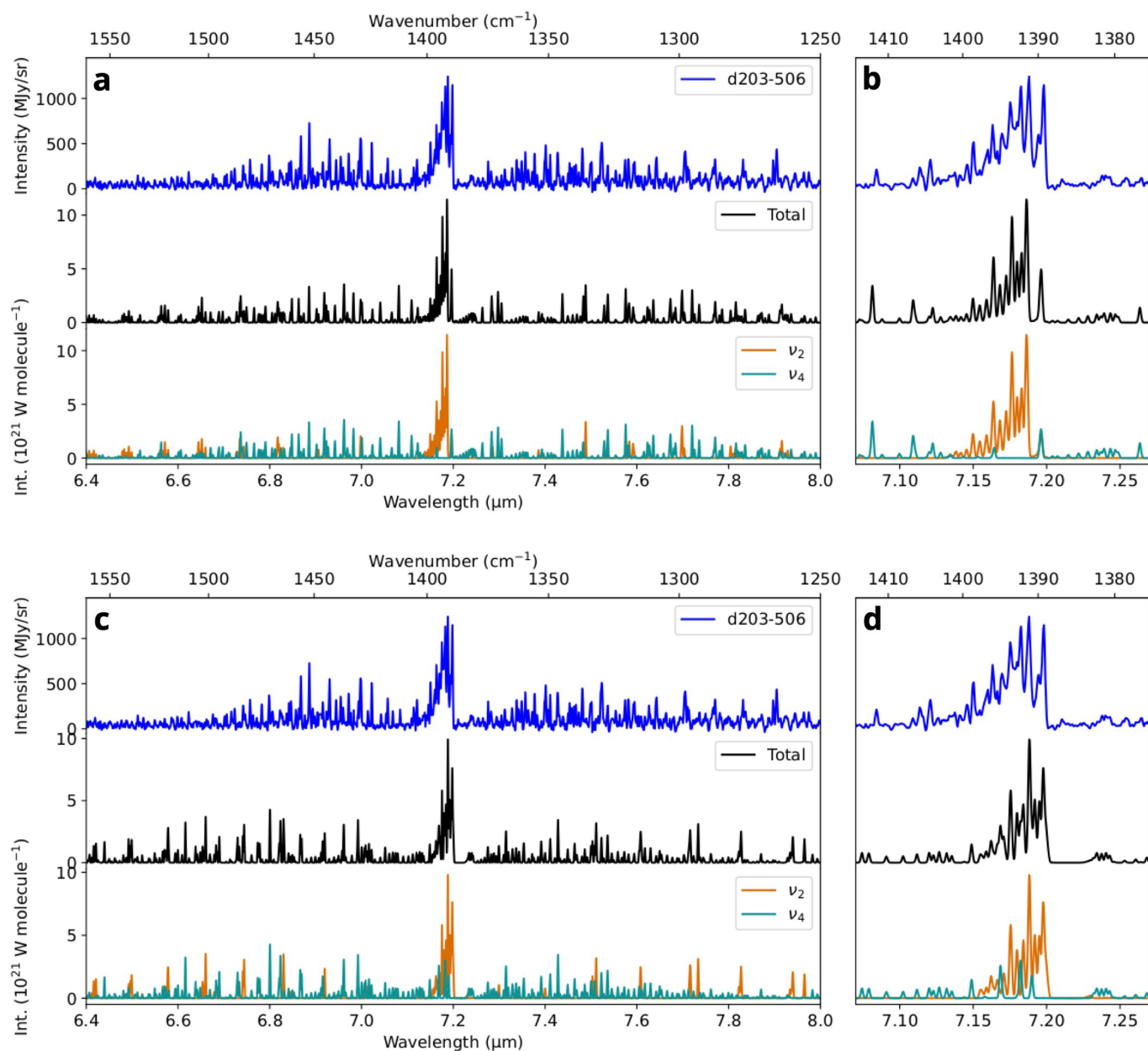
Extended Data Fig. 5 | Spectroscopic models III and IV. a , Model III, with zoom on the strongest lines (b) . c , Model IV, with zoom on the strongest lines (d) . For these models, the excitation temperature is T = 400 K, and we use a Gaussian profile of 0.35 \text{ cm}^{-1} full-width-at-half-maximum.
