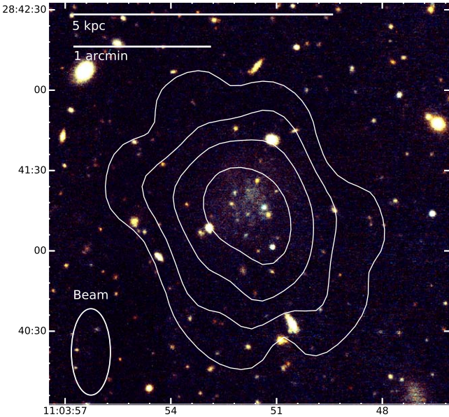
Figure 13. WIYN 3.5 m g' + r' -band composite image of AGC 219369, with WSRT H I column density contours at N_{\text{H I}} = (0.1, 0.5, 1.2, 2.4) \times 10^{20} \text{ cm}^{-2} superimposed in white. The physical scale bar is calculated for a distance of 9.2 Mpc.
