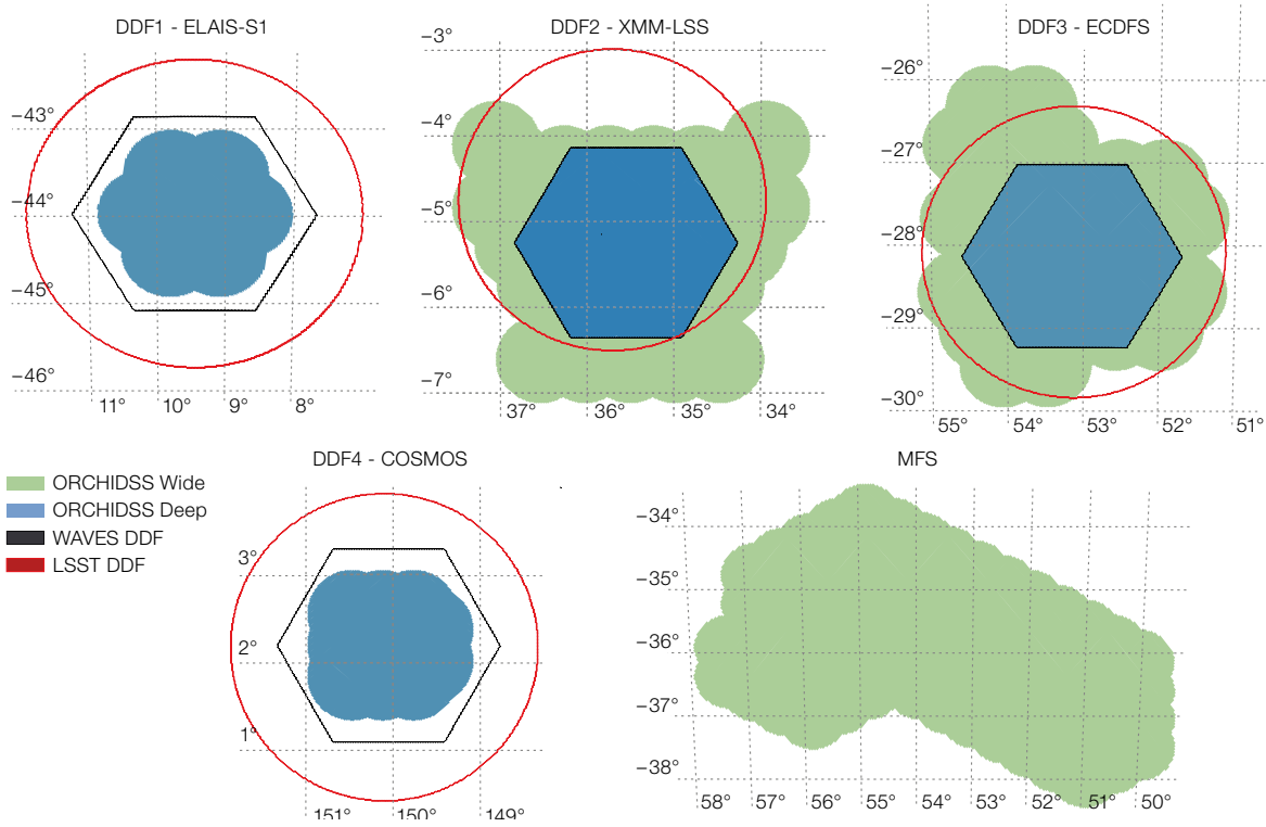
Figure 1. Planned survey fields and maximum potential footprint for the ORCHIDSS Survey. The ORCHIDSS Deep fields (blue shading) align with the WAVES Deep Drilling Fields, targeting MIGHTEE radio-detected sources out to z_{\text{phot}} < 1.4 . ORCHIDSS Wide targets will be drawn from the MIGHTEE and MFS coverage to probe a wider range of cosmic environments out to z_{\text{phot}} < 0.57 .
