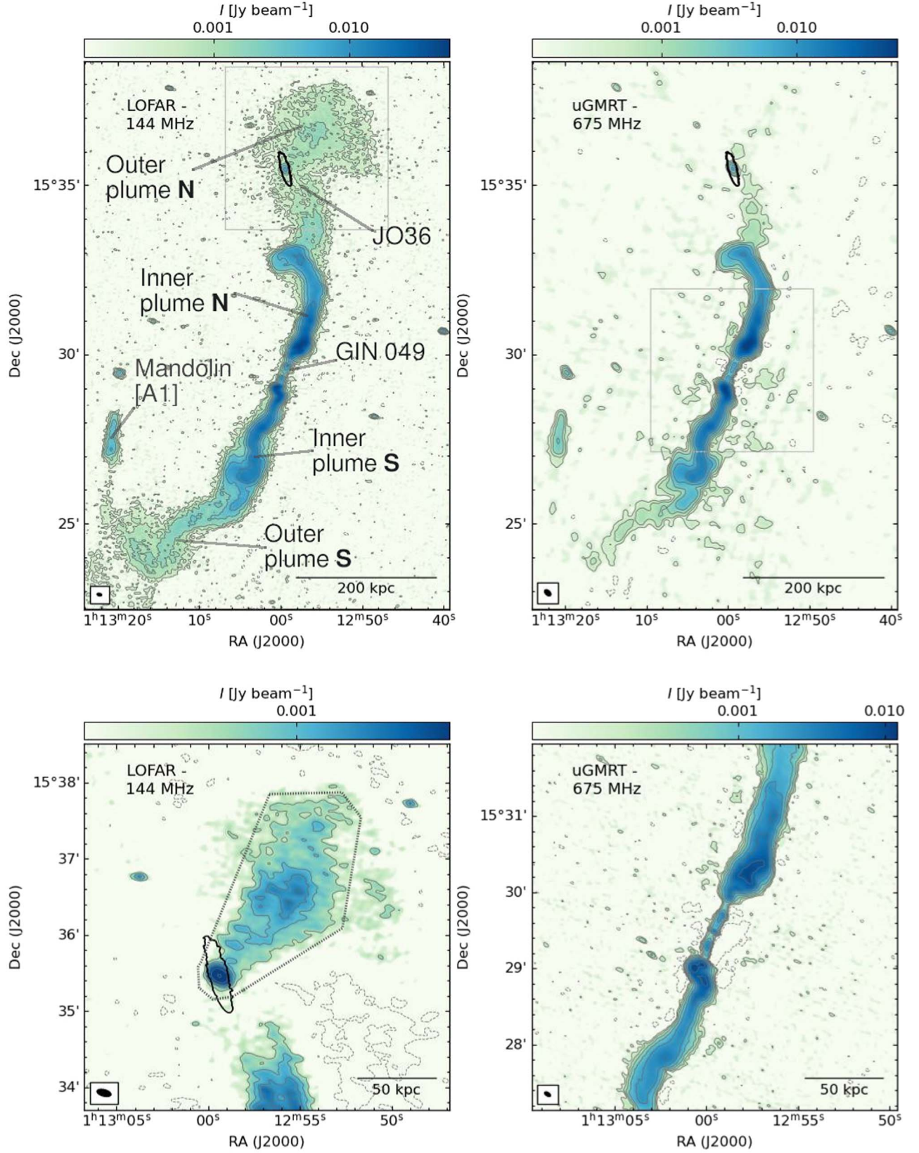
Figure 3. Radio continuum images of the JO36-GIN 049 system. Top-left: 144 MHz ( \text{rms} = 110 \mu\text{Jy beam}^{-1} , resolution = 8.6 \times 4.6 \text{ arcsec}^2 ); top right: 675 MHz ( \text{rms} = 110 \mu\text{Jy beam}^{-1} , resolution = 13.6 \times 8.2 \text{ arcsec}^2 ). Bottom left: 144 MHz ( \text{rms} = 159 \mu\text{Jy beam}^{-1} , resolution = 11.3 \times 5.2 \text{ arcsec}^2 ). The gray-dashed polygon defines the extended region (see Section 3.1). Bottom right: 675 MHz (bottom right, \text{rms} = 40 \mu\text{Jy beam}^{-1} , resolution = 5.4 \times 2.8 \text{ arcsec}^2 ). The relevant parameters used to produce the images with WSCLEAN are reported in Table 1. We show the -3, 3, 6, 12, 24, 48, 96 \times \text{rms} levels (gray), and the contour of the stellar disk of JO36 (black). The silver rectangular regions in the top panels indicate the FOV of the lower panels.
