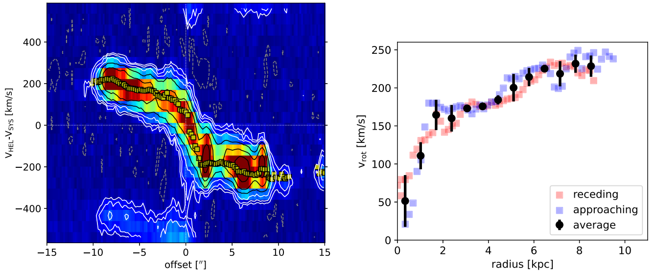
Figure 11. H \alpha kinematics of JO36. Left: position–velocity slice along the galaxy’s major axis, extracted from the MUSE data. The yellow squares show the rotation curve determined with the envelope-tracing method. The bright regions at velocities |v| > 400 \text{ km s}^{-1} are due to the [N II] doublet entering the velocity range of the data cube. Intensity contours are drawn at 3 \times 2^N ( N \geq 0 ) times the rms noise (solid lines). A negative contour at -3 times the rms noise is also shown with gray-dashed lines. Right: the corresponding rotation curve. The approaching and receding sides are shown separately as blue and red squares, respectively. The black circles show the mean rotation velocity.
