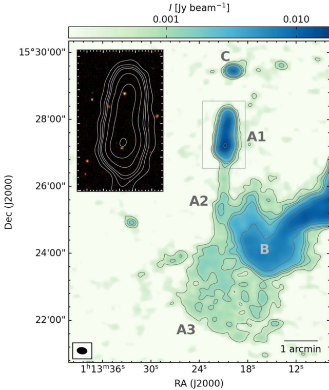
Figure 4. Radio continuum image at 144 MHz of the mandolin radio source with the contours at the 3, 6, 12, 24, 48 \times \text{rms} ( \text{rms} = 172 \mu\text{Jy beam}^{-1} , resolution = 17.7 \times 11.4 \text{ arcsec}^2 ). The labels point out the mandolin (where headstock, neck, and body are, respectively, A1, A2, and A3), GIN 049 southern lobe (B), and WINGS J011319.77+152927.4 (C). In the top-left insert, we show the SDSS optical image of the headstock region (silver box).
