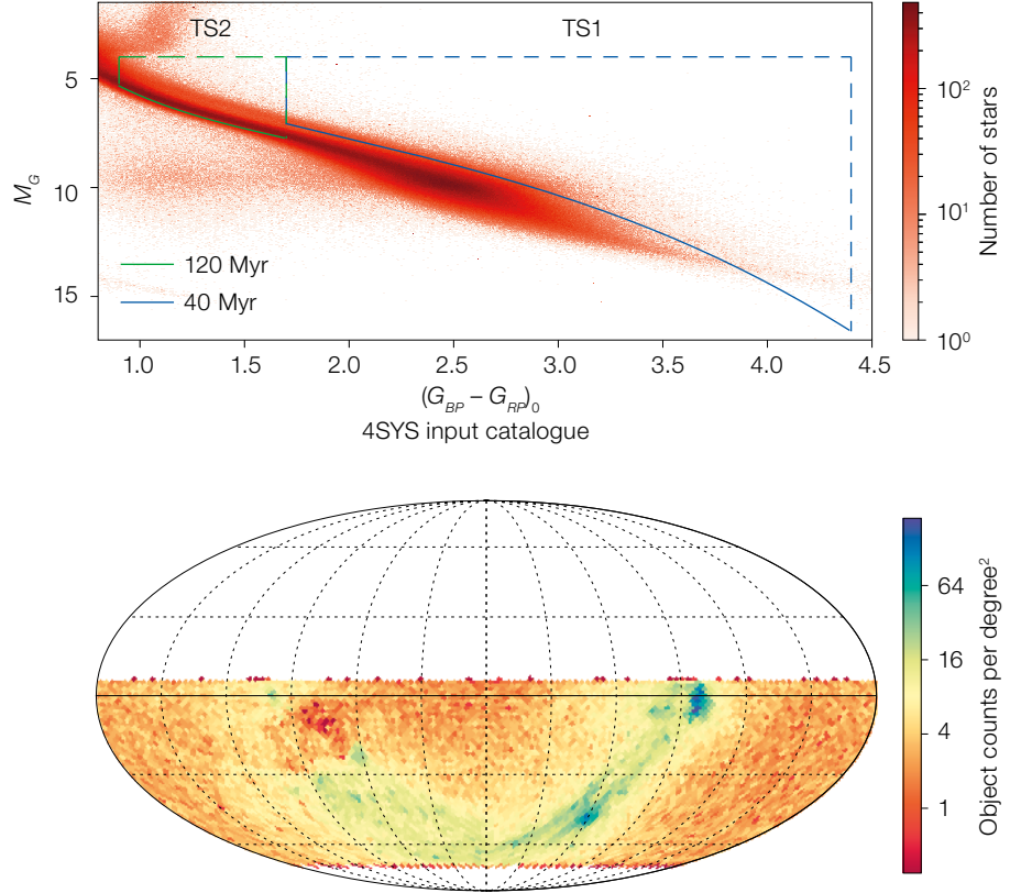
Figure 1. Top panel: two-dimensional histogram representing the absolute G magnitude M_G vs. dereddened (Bp-Rp)_0 colour of all the stars in the Gaia DR3 catalogue with parallax > 2 milliarcseconds, -70 < \text{Declination} < 5 deg, which meet the standard quality criteria for photometry discussed in Riello et al. (2021). The blue and green continuous lines represent the empirical isochrones used to identify stars younger than 40 and 120 Myr, respectively. The areas included within the isochrones and the dashed blue and green lines are used to select stars for the target sample 1 and to pre-select stars for the target sample 2, respectively. Bottom panel: sky distribution of the targets in the 4SYS input catalogue.
