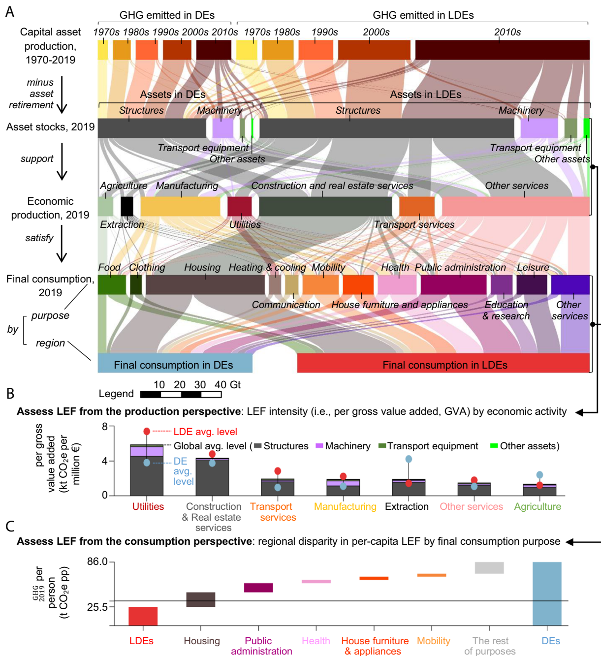
Fig. 3. Mapping LEF 2019 GHG to global production and consumption in 2019. (A) Legacy GHG emissions (LEF 2019 GHG ) mapped to the global value chain by region and sector of production and consumption in 2019. DEs: developed economies; LDEs: less-developed economies (see SI Appendix, Table S1 for countries classified in the DE and LDE regions). Based on the sectoral and regional LEF flows in (A and B) assesses the productive efficiency of capital stocks by normalizing the main economic activities' LEF 2019 GHG by their gross value added in 2019 (adjusted for purchasing power parity), and (C) attributes LEF 2019 GHG to final consumption purposes and population in DEs and LDEs; the horizontal line marks the global average of 34.0 metric tons of CO 2 e per person.
