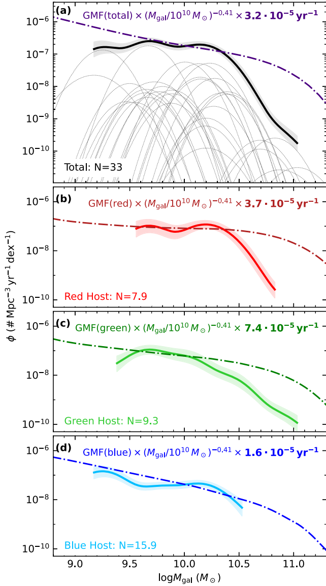
Figure 17. Panel (a): the dotted thin lines represent the values of \mathcal{R}_i (Equation (7)) multiplied by the individual PDFs of \log M_{\text{gal}} . The solid thick black curve shows the total optical TDE rate as a function of M_{\text{gal}} , plotted between the peak of the PDF of the lowest galaxy mass ( 10^{9.17} M_{\odot} ) and highest galaxy mass ( 10^{11.03} M_{\odot} ). The semitransparent region represents the 1\sigma uncertainties. Panels (b)–(d): the observed optical TDE galaxy mass functions in three bins of \mathcal{C} (Equation (23)). The dashed–dotted lines show the local GMFs multiplied by M_{\text{gal}}^{-0.41} and scaled to match the observation at M_{\text{gal}} = 10^{10} M_{\odot} .
