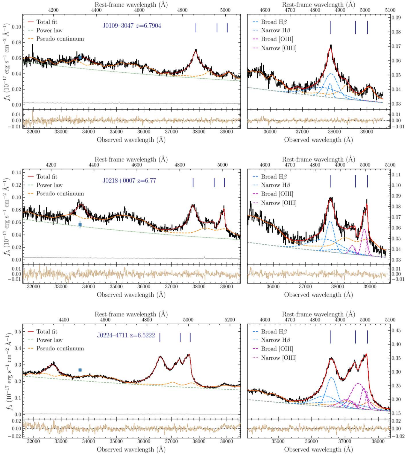
Figure 1. The JWST NIRCcam WFSF F356W spectra of eight ASPIRE quasars (black line) with spectral uncertainty (gray), ordered by R.A. The red solid lines denote the best total fits. The best fits of different spectral components are shown with dashed and dotted lines. For each object, the left panel presents the entire spectrum with total fit, power-law continuum, and pseudocontinuum (i.e., power-law plus Fe II emission). The right panel shows the zoomed-in region of H \beta and [O III] lines. The systemic redshifts of the quasars are based on their [C II] line measurements from ALMA observations. The blue squares with error bars are the photometric data in the WISE W1 3.4 \mu m band. The panels below the spectra present the residuals (data minus model) of each best-fit model.
