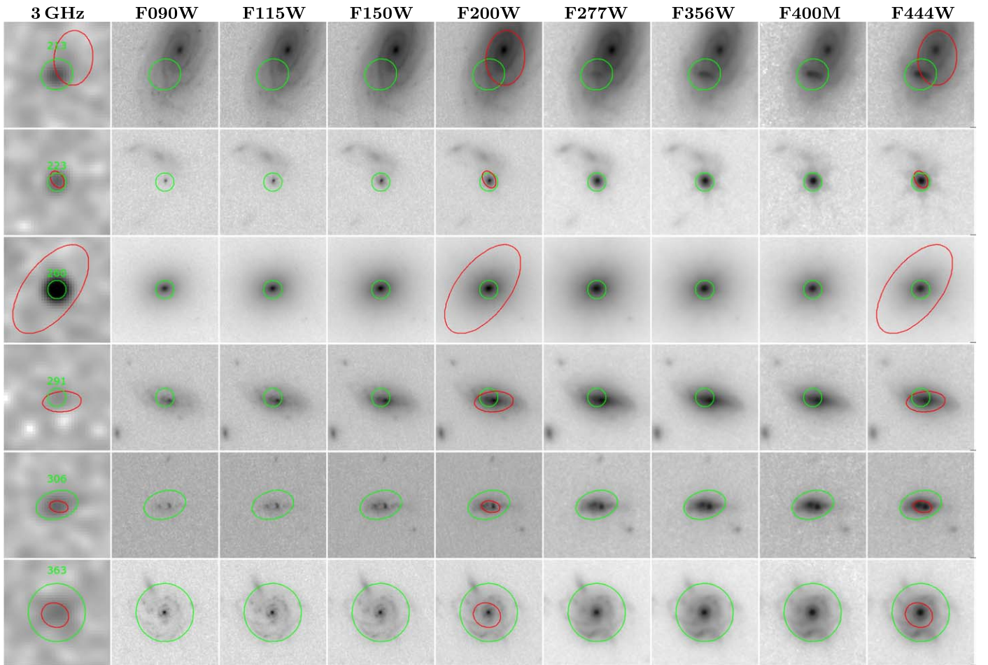
Figure 2. Negative images of six interesting sources. Leftmost panels show the 3 GHz radio image with the source ID included. Other panels show the NIRC images in order of wavelength as labeled at the top. Each thumbnail is 4'' on a side with north up, east to the left. Radio images are all on the same grayscale ( -3 to +35 \mu\text{Jy beam}^{-1} ) and are before primary-beam correction to give nearly constant noise. NIR images have different grayscales for each source, but all images for a given source have the same grayscale to show color information. Green circles or ellipses show the radio positions and radio source sizes (Hyun et al. 2023). Red ellipses show F444W source parameters from SExtractor. (MAG_AUTO photometry ellipses are about 2.5 times larger than the ellipses shown.)
