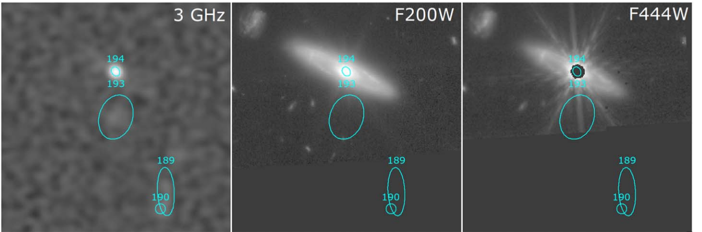
Figure 3. Wider-field images of ID 193. The radio image is on the left, and the other panels show two NIRC images as labeled. The field of view is 16'' in all panels. Ellipses show positions and sizes of four radio sources, the southern two of which are outside the NIRC coverage. The ID 194 nucleus is saturated in the original NIRC data and therefore appears black.
