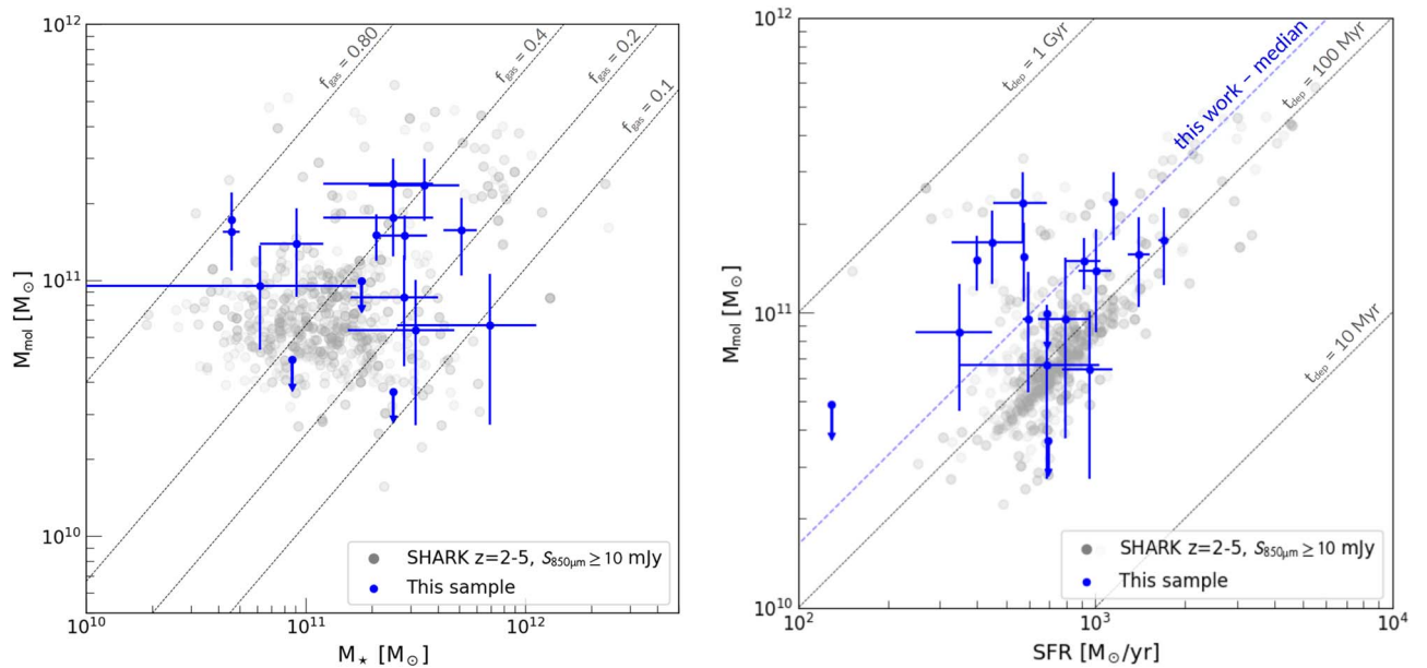
Figure 12. Comparison of our sample with SHARK z = 2-5 SMGs with S_{850\mu} \geq 10 mJy. In the M_* – M_{\text{mol}} plane (left), our observations yield M_{\text{mol}} on the upper end of the SHARK distribution. The SFR– M_{\text{mol}} plane (right) reveals a clear discrepancy in molecular gas depletion timescale t_{\text{dep}} : while SHARK assumes a fixed t_{\text{dep}} = 100 Myr in the starburst mode (notice the conspicuous diagonal trend in the model points), we find a median t_{\text{dep}} = 140 Myr. Despite this limitation, we find a good agreement with our observations, which show a median of \approx 140 Myr.
