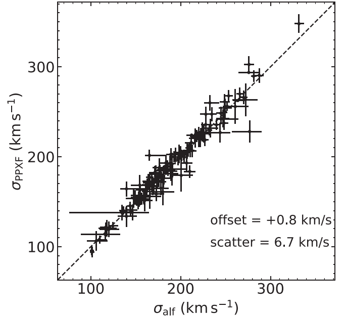
Figure 3. Comparison between velocity dispersions from alf (this study) and from PPXF (reported by the LEGA-C team). Both methods use full-spectrum modeling, but with different underlying stellar libraries. The two methods are in good agreement.
