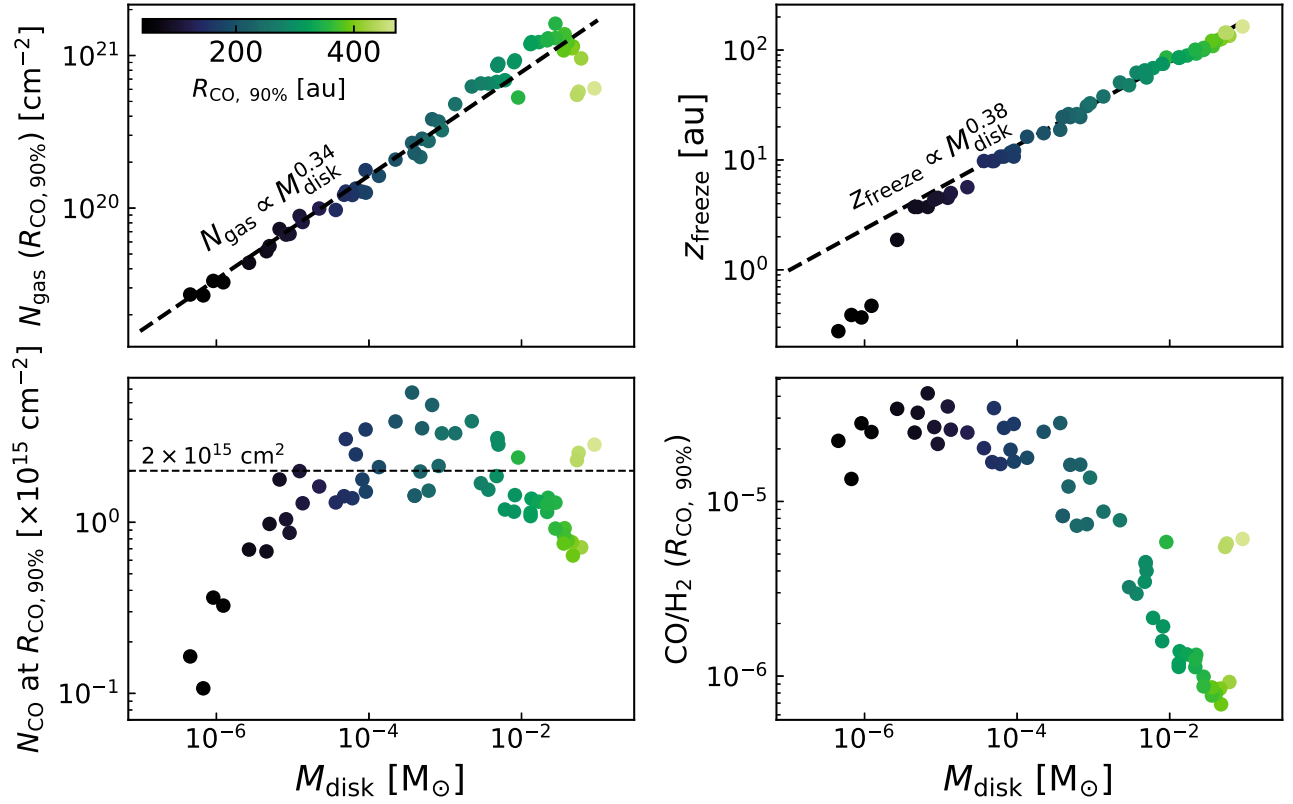
Figure 1. Properties measured at R_{\text{CO},90\%} from DALI models with R_c = 65 au and M_{\text{disk}} = (10^{-7} - 10^{-1} M_{\odot}) . Top left: gas column density at R_{\text{CO},90\%} against the disk mass. Colors show the R_{\text{CO},90\%} of the disk. The black dashed line shows the correlation between N_{\text{gas}}(R_{\text{CO},90\%}) and M_{\text{disk}} . Top right: the height of the CO freeze-out layer at R_{\text{CO},90\%} vs. the disk mass. The black dashed line shows the correlation between z_{\text{freeze}}(R_{\text{CO},90\%}) and M_{\text{disk}} , similar to the one seen in the top-left panel. Bottom left: CO column density at R_{\text{CO},90\%} vs. the disk mass. Bottom right: column-averaged CO abundance (i.e., N_{\text{CO}}(R_{\text{CO},90\%})/N_{\text{gas}}(R_{\text{CO},90\%}) ) at R_{\text{CO},90\%} vs. disk mass.
