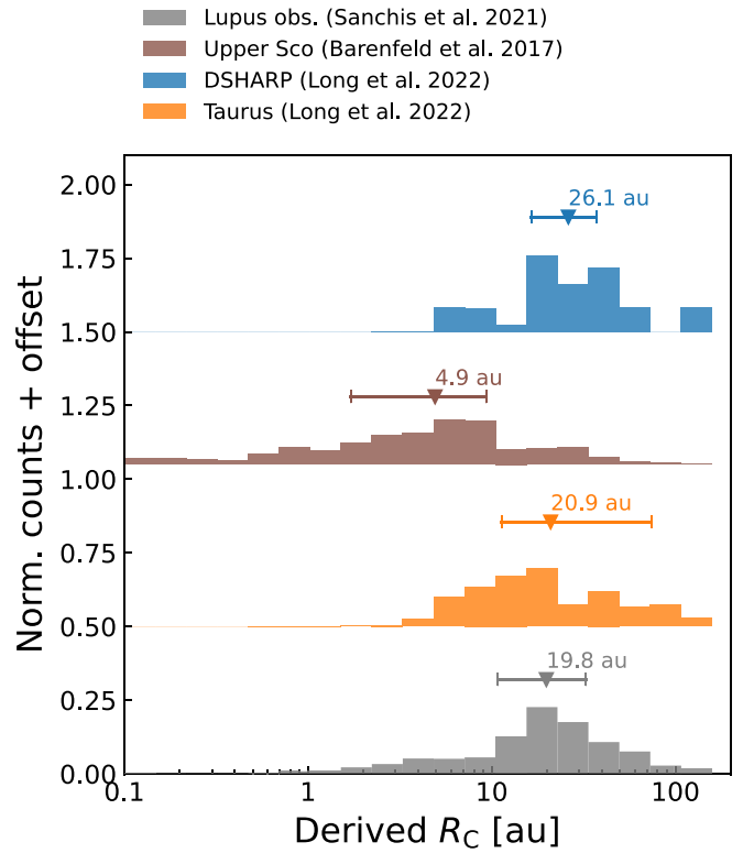
Figure 7. Derived distributions of R_c for four disk samples: Lupus (gray; Andsell et al. 2018; Sanchis et al. 2021), Upper Sco (brown; Barenfeld et al. 2017), Taurus (orange; Long et al. 2022), and DSHARP (blue; Andrews et al. 2018; Long et al. 2022). The triangles denote the median R_c and the horizontal line shows the 25th and 75th quantiles of the R_c distribution of each region. See Table 2 for the R_c of individual disks.
