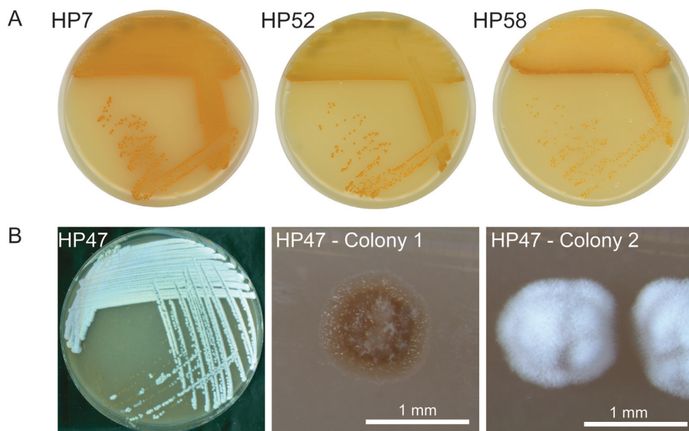
Supplementary Figure 1. Morphology of Micromonospora and Pseudonocardia isolates
