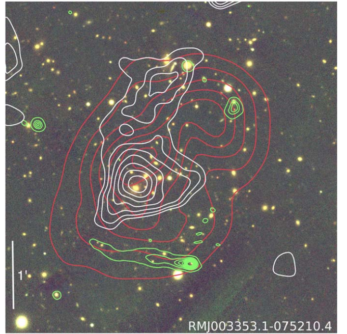
Figure 5. Surface mass density contours from weak lensing (white) overlaid on a Pan-STARRS multiband image and red XMM-Newton surface brightness contours. The small closed contour between the subclusters is a trough. Green GMRT 650 MHz contours (Section 6) start at 70 \mu\text{Jy beam}^{-1} with increments of 680 \mu\text{Jy beam}^{-1} and a 4'' beam.
