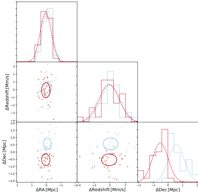
Figure 4. Corner plot showing distribution of subcluster members in R.A., decl., and velocity space relative to the overall mean. Members of the north (south) subcluster are shown in blue (red).
