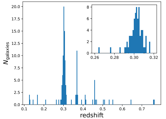
Figure 2. Redshift histogram, with inset showing the redshift interval around A56.
