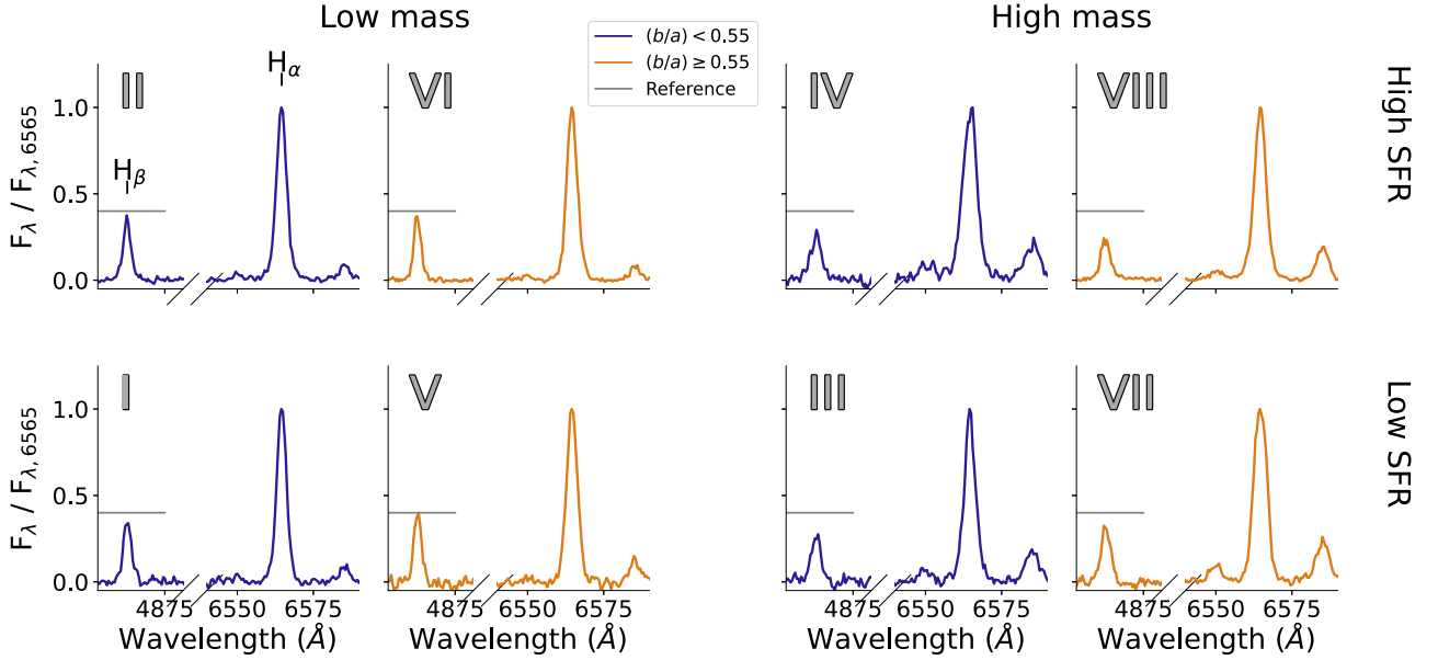
Figure 4. Stacked spectra for the eight groups illustrated in Figure 1. We organize the spectra by stellar mass (left: low mass, right: high mass), SFR (bottom: low SFR, top: high SFR), and axis ratio (blue: edge-on, orange: face-on). The continuum has been subtracted for all stacked spectra. The spectra are normalized so they have the same H \alpha peak flux for visual comparison. It is visible that the lower-mass galaxies (left) have higher normalized H \beta fluxes than the higher-mass galaxies (right), which results in a smaller Balmer decrement for the lower-mass galaxies. We do not observe a clear change in the Balmer decrement with a changing axis ratio for any of the groups.
