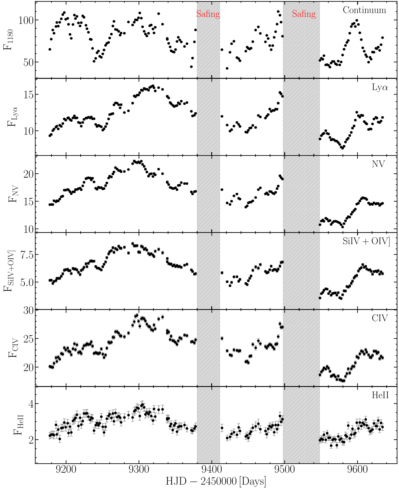
Figure 4. Integrated continuum light curve at 1180 Å (top panel) and emission-line light curves for \text{Ly}\alpha , NV, Si IV + IV blend, CIV, and He II, respectively, in panels below the top panel. The \text{Ly}\alpha light curve is the integrated flux in the blue wing of the emission line over the region not contaminated by absorption, and thus only includes 21% of the total emission-line profile (see Table 2). All the light curves are computed from the observed-frame spectra. The continuum light curve is in units of 10^{-15} \text{ erg s}^{-1} \text{ cm}^{-2} \text{ Å}^{-1} and the line fluxes are in units of 10^{-13} \text{ erg s}^{-1} \text{ cm}^{-2} . The hashed gray regions display the two major observation gaps during our campaign, which were the result of HST safing events.
