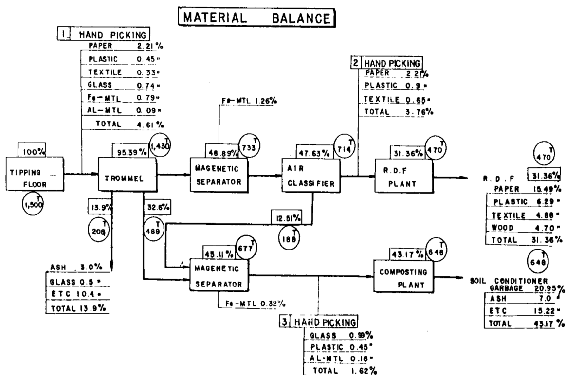
Figure 1-8 Waste treatment plant operation process
