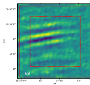
Figure 2.15: Artefact within the 100 morphological outliers.
