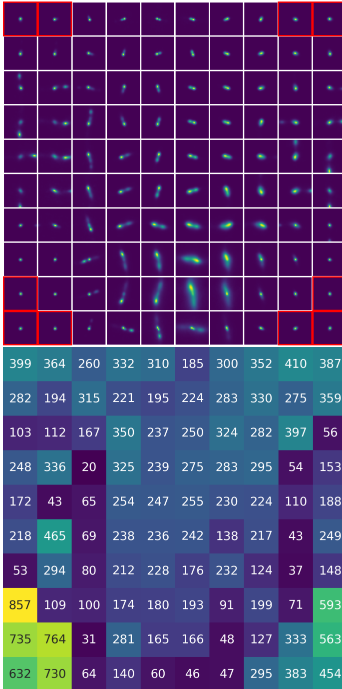
Figure 2.13: Top panel : First run 10 \times 10 cyclic SOM. The first run reveals that our preprocessed dataset still contains a large fraction of unresolved sources. We remove these from the training dataset by removing all radio sources that map to one of the red highlighted representative images. Bottom panel : Heatmap of the first run SOM, indicating the number of sources mapped to each of the representative images.
