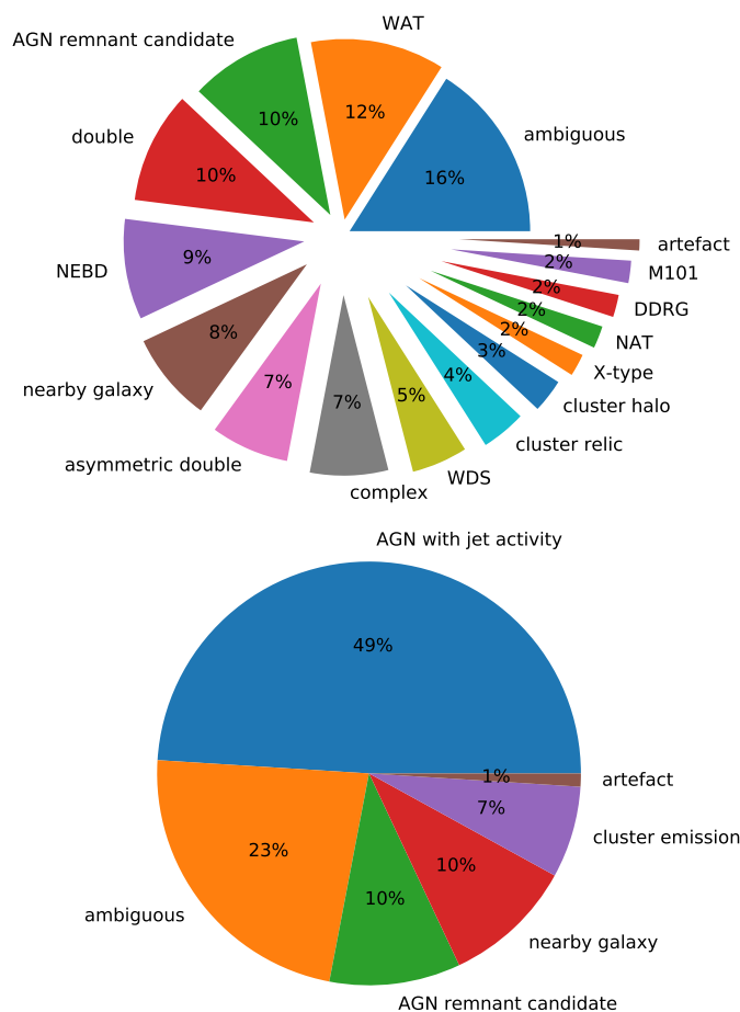
Figure 2.11: Piechart showing the wide variety of morphologies and radio source types present in the 100 most outlying sources in the final 10 \times 10 cyclic SOM. Top panel: Descriptive labels have been established by a manual visual inspection of each source in radio (LoTSS), mid-infrared (WISE) and optical (SDSS 9 colour). We labelled sources that fitted in more than one category as ‘ambiguous’. ‘X-type’ sources are ‘X-shaped’ extended doubles (Rees, 1978), ‘WATs’ and ‘NATs’ are Wide Angle Tailed and Narrow Angle Tailed sources, ‘WDS’ are Wide Double Sources, ‘NEBD’ are Narrow Edge Brightened Doubles (Miley, 1980), ‘DDRGR’ are Double-Double Radio Galaxies (Schoenmakers et al., 2000). An ‘AGN remnant candidate’ is an extended double with such relaxed morphology that the AGN jets might not be active any more. As M101 is an exceptionally large apparent object, the source detection software did not group the separate detections of this nearby spiral, as a result it features multiple times in the catalogue. Bottom panel: We grouped subtypes together to get an overview of the dominant types of sources in the outliers: ‘M101’ was grouped with ‘nearby galaxy’, ‘complex’ with ‘ambiguous’, ‘cluster relic’ and ‘cluster halo’ were grouped into ‘cluster emission’ and ‘DDRGR’, ‘NEBD’, ‘NAT’, ‘WAT’, ‘WDS’, ‘double’, ‘asymmetric double’ and ‘X-type’ were grouped into ‘AGN with jet activity’. A figure containing each of these one hundred most outlying sources can be found in Appendix 2.B.
