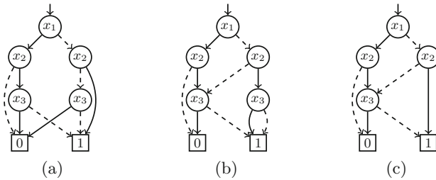
Fig. 1. (Ordered) BDDs representing function f = (x_1 \wedge x_2 \wedge \overline{x_3}) \vee (\overline{x_1} \wedge \overline{x_2} \wedge \overline{x_3}) \vee (\overline{x_1} \wedge x_2 \wedge x_3) . For node v , we draw \text{var}(v) = i as x_i . Dashed lines represent low branches ( v[0] ) and solid lines high branches ( v[1] ). Only the BDD in (c) is completely reduced. The BDD in (a) can be reduced to (c) by merging the two isomorphic nodes for x_3 , while the BDD in (b) can be reduced to (c) by removing the (right-most) redundant node x_3 .
