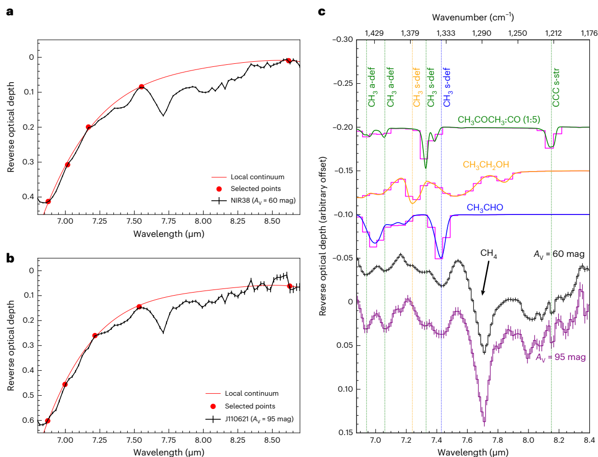
Fig. 3 | Detections of COM functional groups. a,b , Local continuum over the optical depth spectra of NIR38 ( A_V = 60 mag; a ) and J110621 ( A_V = 95 mag; b ) in the range between 6.9 \mu\text{m} and 8.6 \mu\text{m} . c , Local continuum subtracted spectra of NIR38 ( A_V = 60 mag) and J110621 ( A_V = 95 mag) compared with laboratory infrared spectrum of COMs ( \text{CH}_3\text{CHO} , green line 31 ; \text{CH}_3\text{CH}_2\text{OH} , orange line 31 ;
