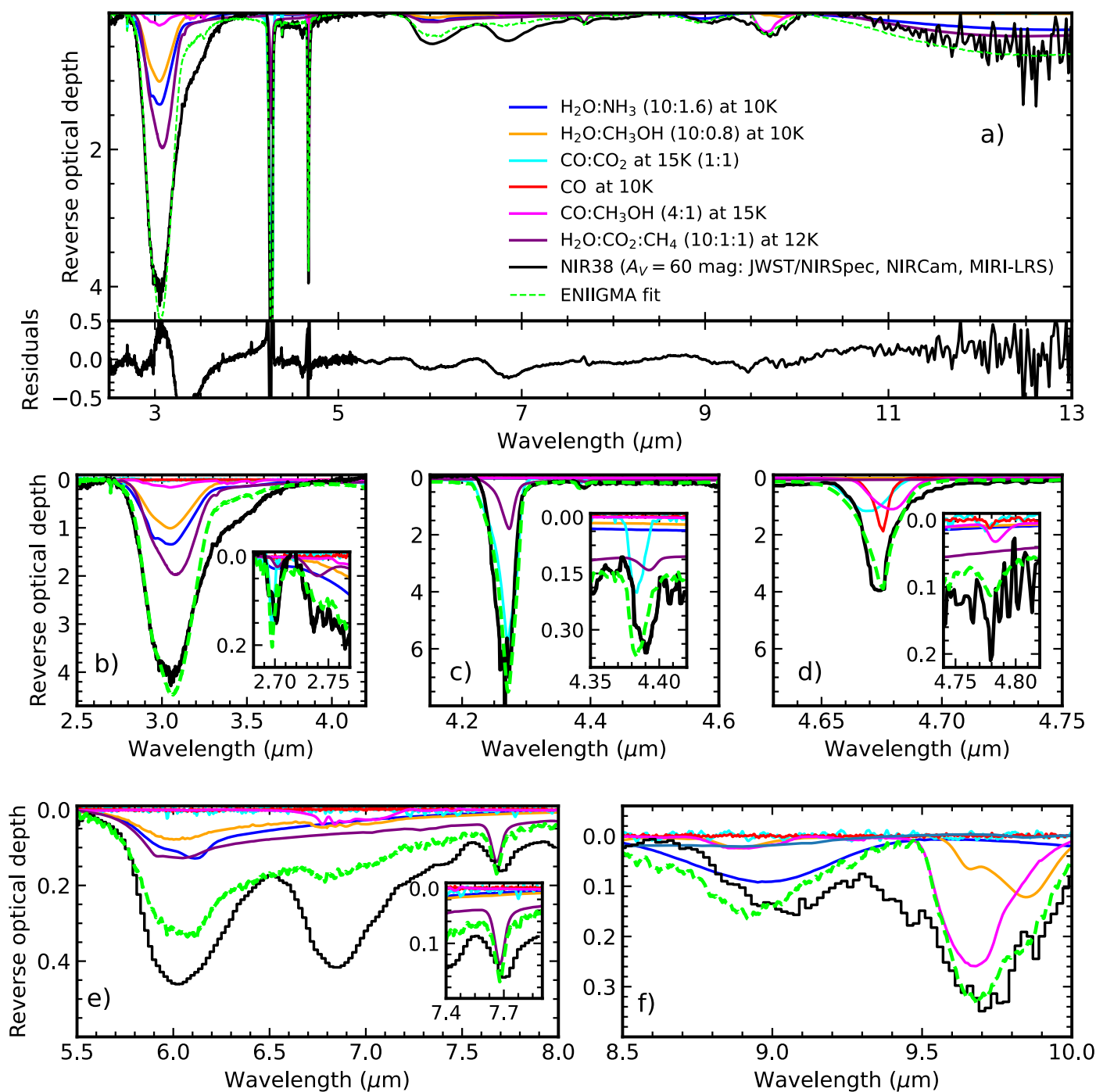
Extended Data Fig. 1 | Global fit of the combined spectrum for NIR38.
