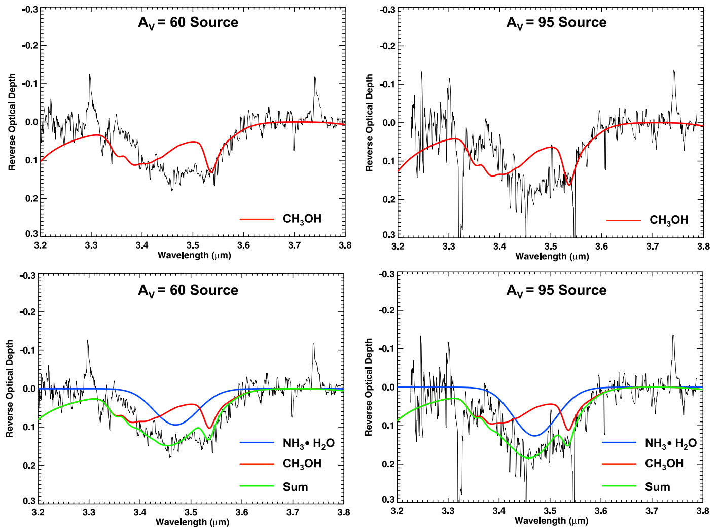
Extended Data Fig. 9 | Optical depths of the A_V = 60 mag (NIR38, left) and A_V = 95 mag (J110621, right) background sources in the 3.2 – 3.8 \mu\text{m} ( 3125 – 2631 \text{ cm}^{-1} ) region. Top: The red line shows the optical depths of \text{CH}_3\text{OH} laboratory data at 15K scaled for the C–H stretching band around the 3.53 \mu\text{m}
