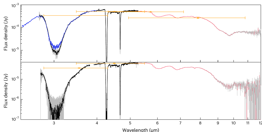
Fig. 2 | Data quality comparison for NIR38 and J110621. Top: comparison of the NIRCam WFSS (blue), NIRSpec FS (black) and MIRI LRS FS (red) spectra of the A_V = 60 mag background star. Error bars (grey) are 3\sigma , and in some regions are smaller than the thickness of the lines. Spitzer IRAC photometry (gold points)
