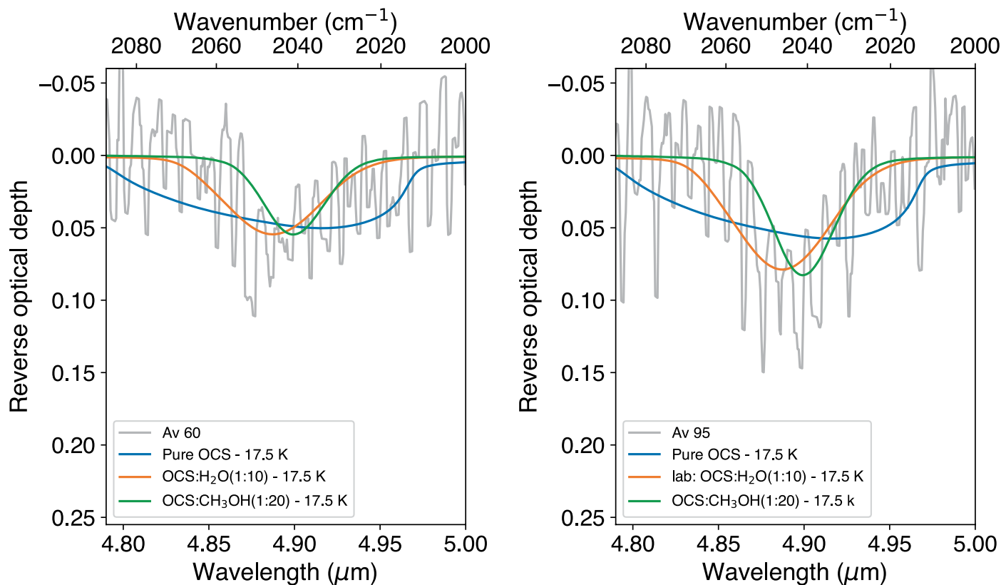
Extended Data Fig. 8 | Observed absorption profile of the C=O stretching of OCS, around 4.9 μm, towards NIR38 (left panel) and J110621 (right panel). The coloured curves show the profile of the OCS in laboratory ice spectra of pure OCS (blue), H 2 O:OCS (orange), and CH 3 OH:OCS (green), all at 17.5 K.
