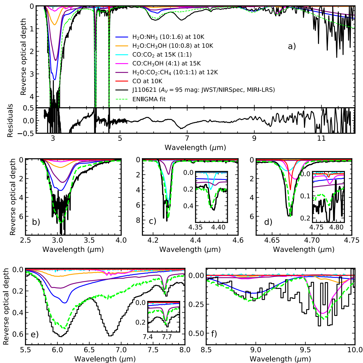
Extended Data Fig. 2 | Global fit of the combined spectrum for J110621.
