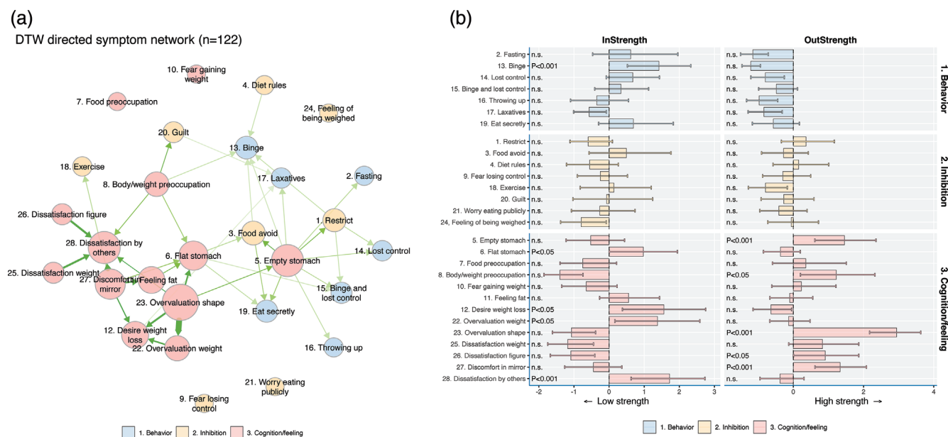
FIGURE 2 (a) Directed EDE-Q symptom network. (b) Standardized centrality values.
