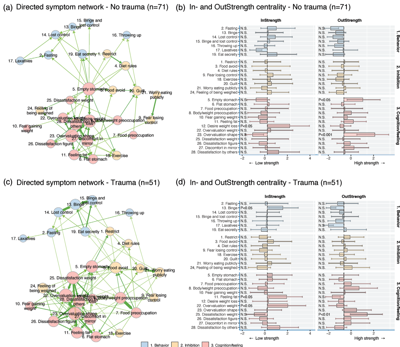
FIGURE 3 (a-d) Directed symptom network for patients with and without childhood maltreatment.
