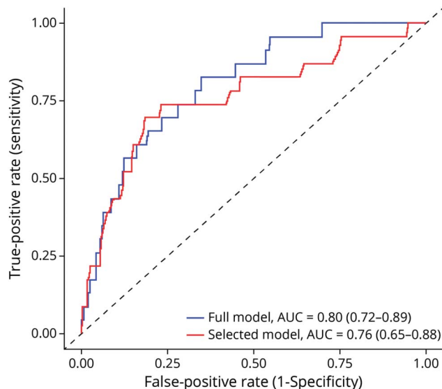
Figure 1 ROC Curve for Predicted Probability of Finding an Unruptured Intracranial Aneurysm at Screening
