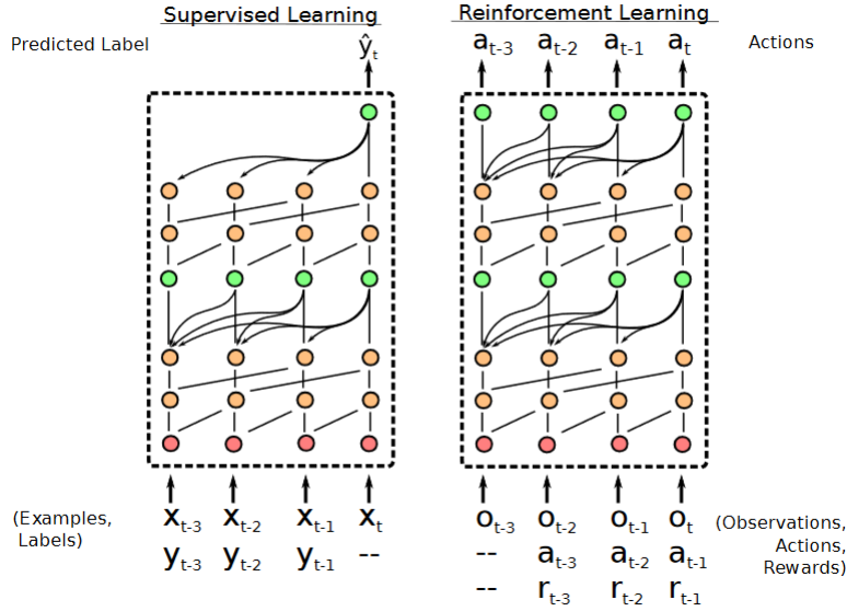
Figure 2.17: Architecture and workflow of SNAIL for supervised and reinforcement learning settings. The input layer is red. Temporal Convolution blocks are orange; attention blocks are green. Source: Mishra et al. (2018).
