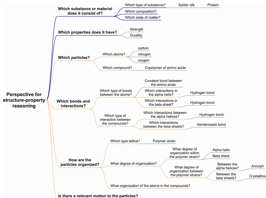
Fig. 7 Elaborated perspective for structure–property reasoning for the case of spider silk
