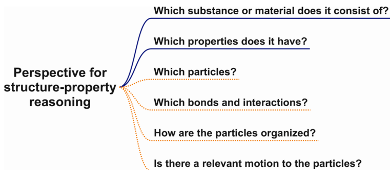
Fig. 2 The six main questions of the perspective for structure–property reasoning: dark blue lines for the macro-level questions, dotted orange lines for the micro-level questions
