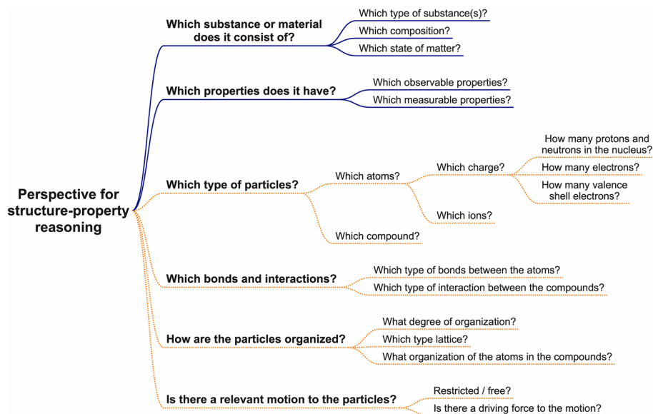
Fig. 3 The perspective for structure–property reasoning elaborated with several levels of questions: dark blue lines for the macro-level questions, dotted orange lines for the micro-level questions
