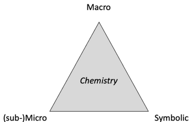
Fig. 1 Johnstone triangle (adapted from Reid, Norman. “A tribute to Professor Alex H Johnstone (1930–2017): His unique contribution to chemistry education research” Chemistry Teacher International , vol. 1, no. 1, 2019, pp. 20,180,016.)
