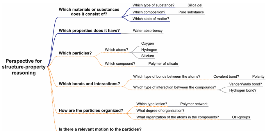
Fig. 5 Elaborated perspective for structure–property reasoning for the case of silica gel
