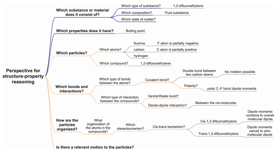
Fig. 6 Elaborated perspective for structure–property reasoning for the case of cis–trans isomerism
