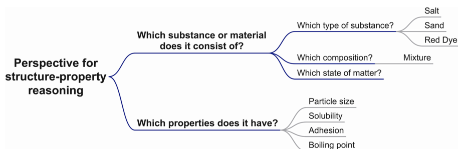
Fig. 4 Elaborated perspective for structure–property reasoning for the case of separation methods
