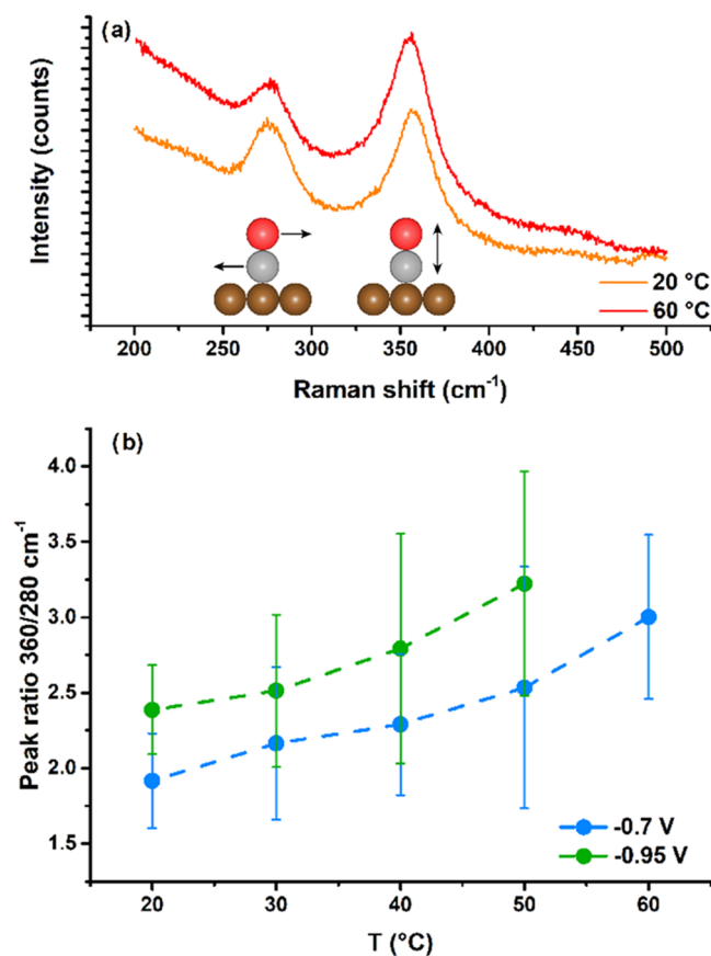
Figure 3. (a) Unprocessed Raman spectrum at 20 and 60 °C and −0.7 V vs RHE, representative for the other Raman spectra. (b) Ratio between the 360 and 280 cm −1 Raman peak areas on Cu in 0.1 M KHCO 3 as a function of reaction temperature, at −0.7 and −0.95 V vs RHE. The error bars are composed of at least 4 spectra, and the dotted lines are a guide to the eye.
