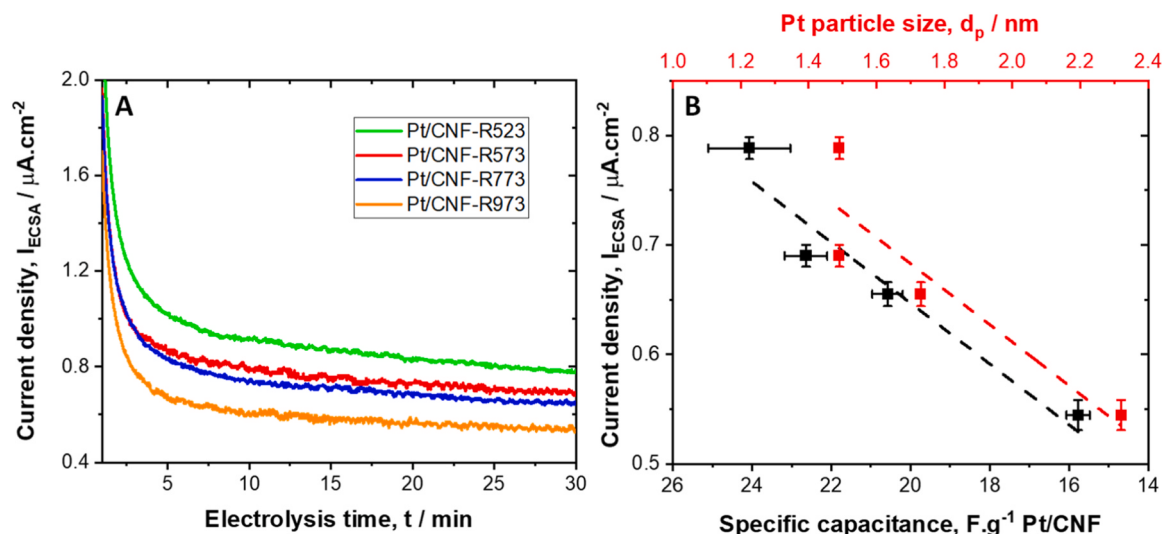
Fig. 6. A) Background-corrected current densities measured in 0.1 M H_2SO_4 in the presence of 0.1 M glucose at 0.78 V vs. RHE and B) the corresponding current density measured after 30 min chronoamperometry as a function of the specific capacitance ( R^2 = 0.91 ) and Pt particle size ( R^2 = 0.76 ) of the Pt/CNF electrocatalysts.
