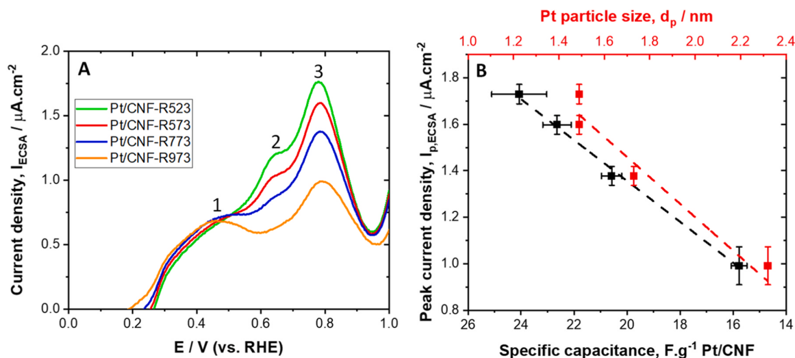
Fig. 5. A) Background corrected linear sweep voltammetry measured in 0.1 M \text{H}_2\text{SO}_4 in the presence of 0.1 M glucose at 1 \text{ mV.s}^{-1} and B) the corresponding peak current density measured by LSV at 0.78 V vs. RHE as a function of the specific capacitance ( R^2 = 0.99 ) and Pt particle size ( R^2 = 0.90 ) of the Pt/CNF electrocatalysts.
