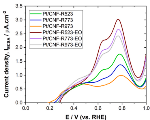
Fig. 8. Background corrected linear sweep voltammetry measured at 1 \text{mV}\cdot\text{s}^{-1} in 0.1 M \text{H}_2\text{SO}_4 and 0.1 M glucose for pristine Pt/CNF-R523, Pt/CNF-R773 and Pt/CNF-R973 and Pt/CNF-R523-EO, Pt/CNF-R773-EO and Pt/CNF-R973-EO.
