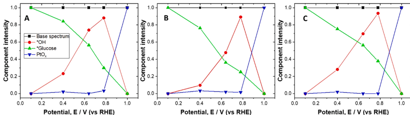
Fig. 7. Results of LCA of HERFD-XANES spectra at Pt L III -edge obtained at various hold potentials in 0.1 M H_2SO_4 and 0.1 M glucose for Pt/CNF-R523 (A), Pt/CNF-R773 (B) and Pt/CNF-R973 (C).
