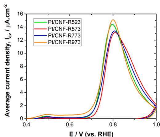
Fig. 3. Background corrected CO-stripping curves corrected for of Pt/CNF catalysts obtained in 0.1 M H 2 SO 4 recorded at 5 mV.s -1 .
