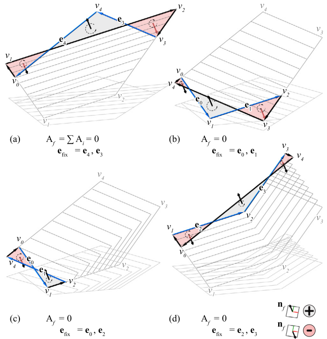
Fig. 10. (a) to (d) Various zero-area computation for a starting face with the area A_f and different chosen fixed edges.
