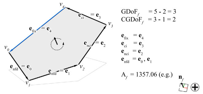
Fig. 7. A sample face showing the edge vectors, its normal direction and the choices of e_{fix} , e_{cr} , e_{nci} , and e_{nfd} .
