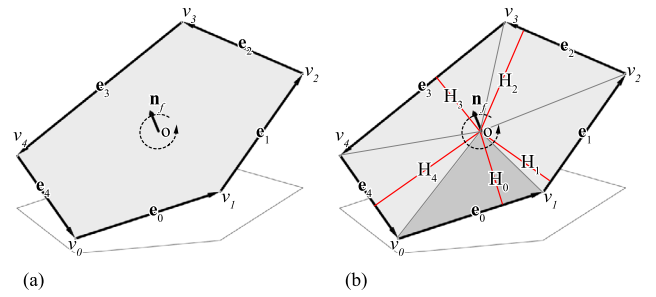
Fig. 5. (a) Vertices and edge vectors of the face f with a normal direction \mathbf{n}_f ; and (b) dividing the face into triangles with a base e_i and the height H_i from the centroid of the vertices.
