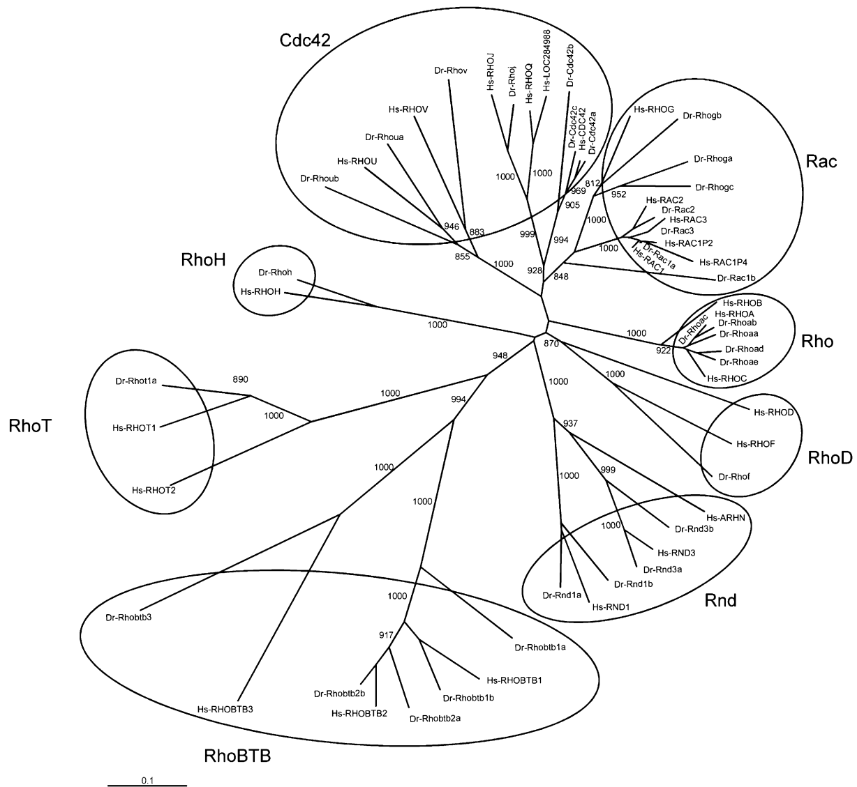
Fig. 3. Unrooted phylogenetic tree of human and zebrafish Rho GTPases. Human proteins are in capitals; zebrafish protein names are in lowercase. The tree was constructed by neighbor-joining analysis based on an alignment of the amino acid sequences of the Rho domains. The numbers indicate the occurrence of nodes during bootstrap analysis with 1000 reiterations. Only values above 800 are shown.
