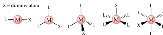
Scheme 1. Schematic Figure to Exemplify Where the Dummy Atom Will Be Positioned if the Metal Center in the Metal–Organic Compound Is Di-, Tri-, Tetra-, Penta-, or Hexa-Coordinated
