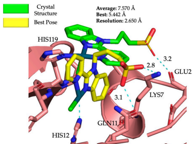
Figure 3. X-ray structure and the best pose of the Pd metal complexes that were used as a validation run. The green structure is the metal complex in the X-ray, the yellow structure is the pose that was obtained with the best RMSD, and the pink residues represent the protein residues that interacted more strongly with the metal–organic compound.
