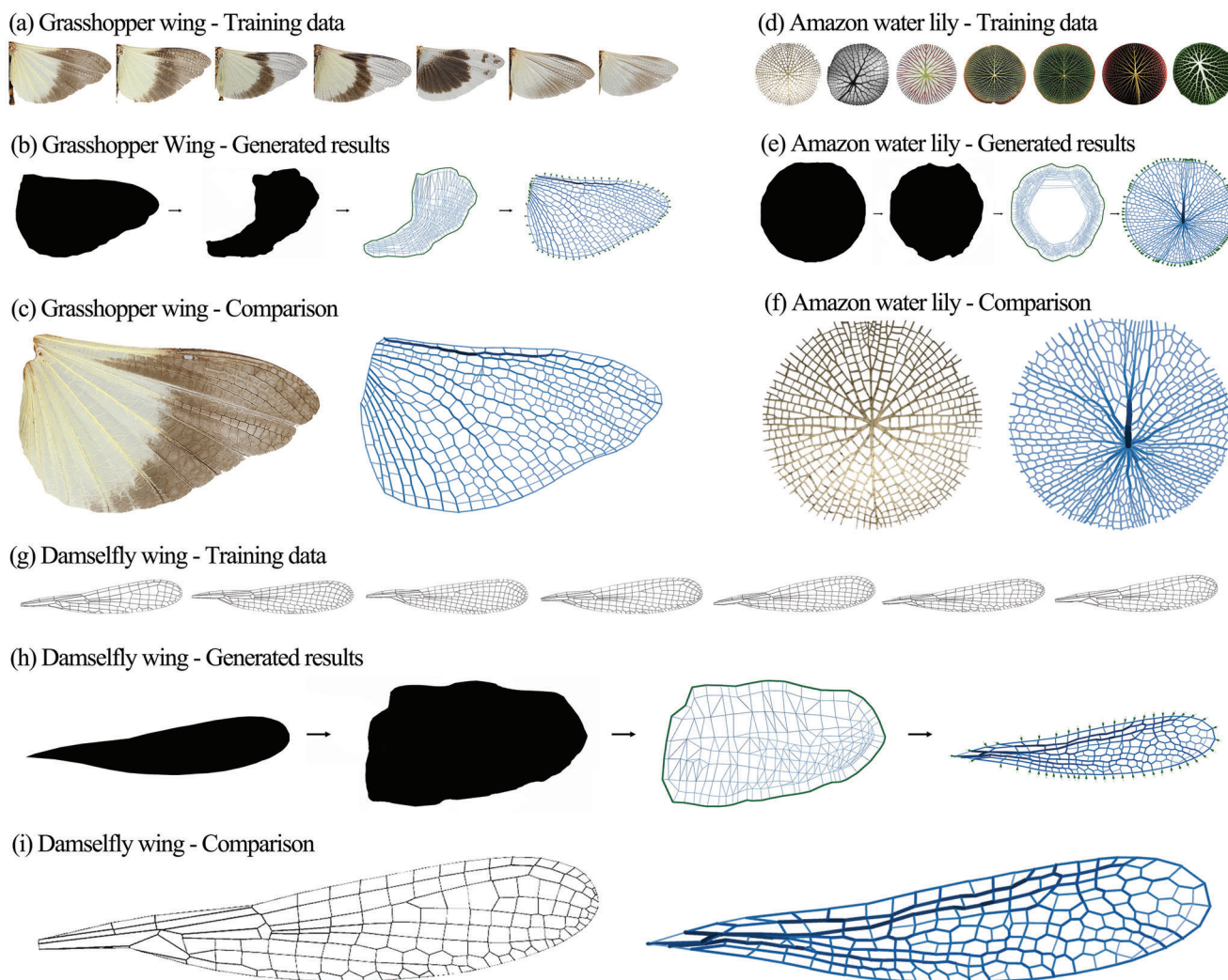
Figure 7. a) Training dataset of the grasshopper wing. b) Generated results of testing data of the grasshopper wing by machine learning. c) Comparison of the real grasshopper wing and the generated structural form. (The virtual loads are not shown.) d) Training dataset of the Amazon water lily. e) Generated results of testing data of the Amazon water lily by machine learning. f) Comparison of the real Amazon water lily and the generated structural form. (The virtual loads are not shown.) g) Training dataset of the damselfly wing. h) Generated results of testing data of the damselfly wing by machine learning. i) Comparison of the real damselfly wing and the generated structural form. (The virtual loads are not shown.)
