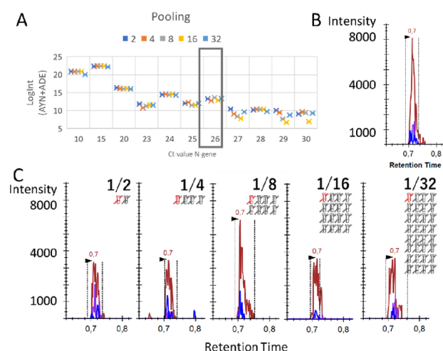
Figure 4. SISCAPA peptide immuno-affinity enrichment is insensitive to patient pooling. (A) 10 \mu L out of 50 \mu L of the peptide digest of positive patient samples with different Ct values were diluted with q-PCR-confirmed negative patient samples in five different ratios (1/2, 1/4, 1/8, 1/16, and 1/32), with each dilution corresponding to a loss of one Ct value ( n = 1 ). However, by using SISCAPA peptide immuno-affinity enrichment, LC–MS is insensitive to the dilution effect; hence, a similar signal intensity is achieved for each dilution. (B) One positive (red) patient with Ct 26 (boxed in (A)) was manually inspected. The initial measurement of 50 \mu L sample resulted in a signal for AYN of 7000. (C) When another 50 \mu L of digest from this patient was split into five and diluted 1/2, 1/4, 1/8, 1/16, and 1/32 with a digest of mixture of negative patients, the signal did not decline accordingly, effectively showing how the SISCAPA workflow is insensitive to pooling.
