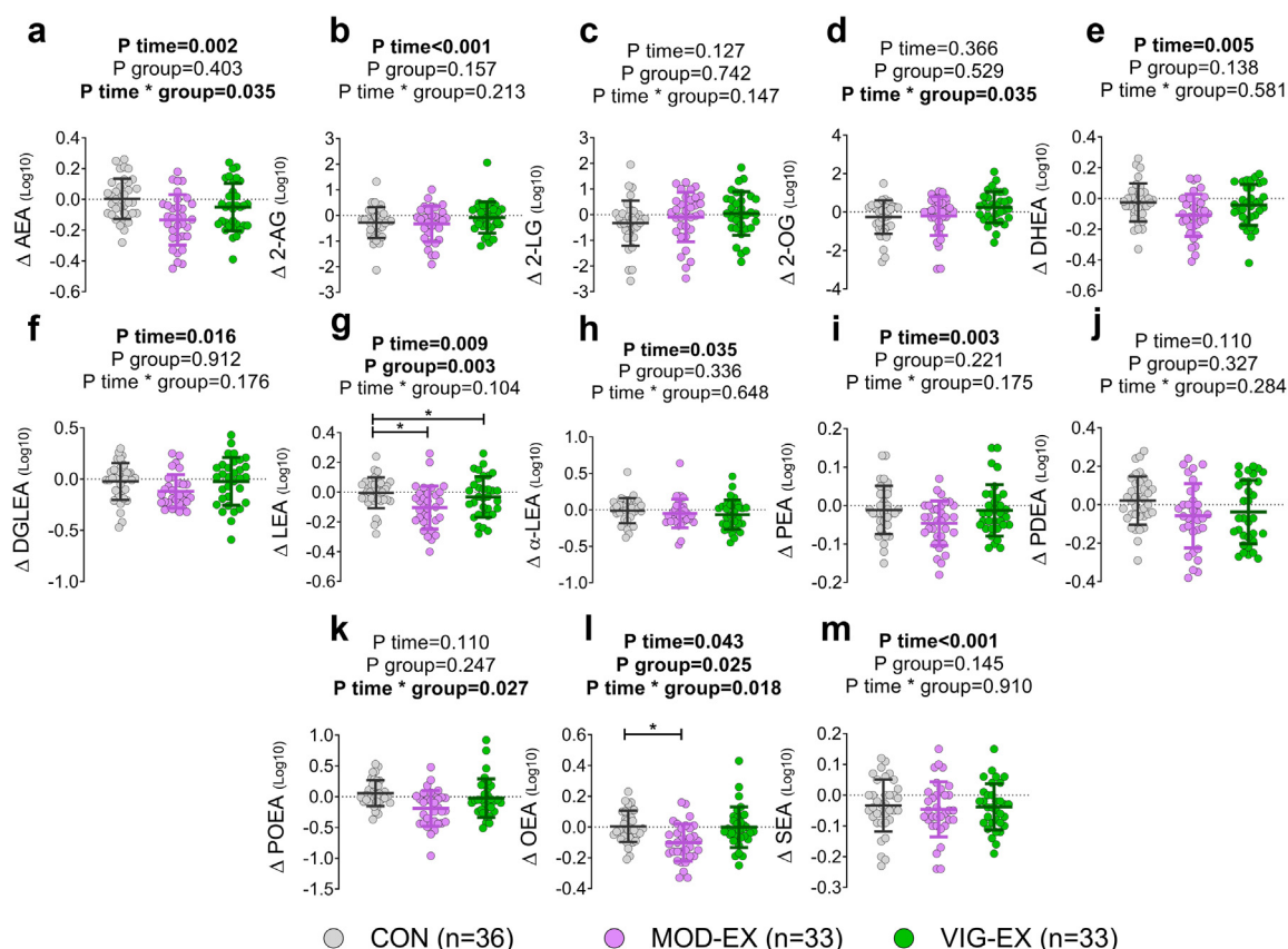
Fig. 5: Long-term moderate, exercise training decreases plasma levels of endocannabinoids analogues in young adults. a–m: Δ was calculated as post minus baseline values of the area peak ratio for each endocannabinoid and analogue. P value obtained from linear mixed repeated measures analyses. Data represent mean and standard deviation. * Symbol means statistically significant differences between groups after posthoc Bonferroni correction. Abbreviations: 2-AG, 2-arachidonylglycerol; 2-LG, 2-linoleoylglycerol; 2-OG, 2-oleoylglycerol; AEA, anandamide; CON, control group; DGLEA, dihomogamma-linolenoyl ethanolamide; DHEA, docosahexaenoyl ethanolamide; LEA, linoleoyl ethanolamide; MOD-EX, moderate-intensity exercise group; OEA, oleoyl ethanolamine; PDEA, pentadecanoyl ethanolamide; PEA, palmitoyl ethanolamide; POEA, palmitoleoyl ethanolamide; SEA, stearoyl ethanolamide; VIG-EX, vigorous-intensity exercise group; α-LEA, α-linolenoyl ethanolamide.
