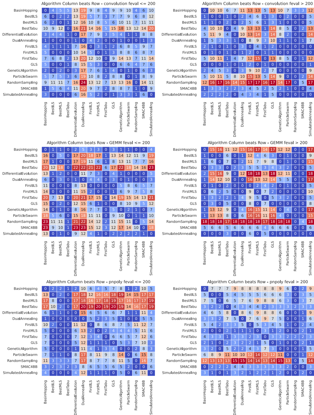
Fig. 1. Heatmaps counting the occurrences when the column algorithm found statistically better solutions than the row algorithm for the (top) convolution, (middle) GEMM, and (bottom) PnPoly kernels. An occurrence is counted when 50 runs for a budget are statistically significantly better according to a two-sample independent t -test ( \alpha = 0.05 ). (Left): Heatmap for low \leq 200 budgets, i.e., 25, 50, 100, and 200. (Right): Heatmap for mid and high > 200 budgets, i.e., 400, 800, and 1600. Algorithms with low values (blue) in their rows were not often beaten for those budgets, and algorithms with high values in their column (red) often beat other algorithms.
