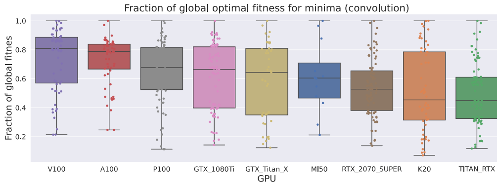
Fig. 3. Fraction of optimal fitness of local minima for each GPU model, for the convolution kernel. The box plots shows the median line, the box designates the quartiles, and the whiskers designates the full extend of the distribution. Additionally, a scatter plot of the fitness for each local minimum is shown. The GPUs are ordered in descending median fraction of optimal fitness from left to right.
