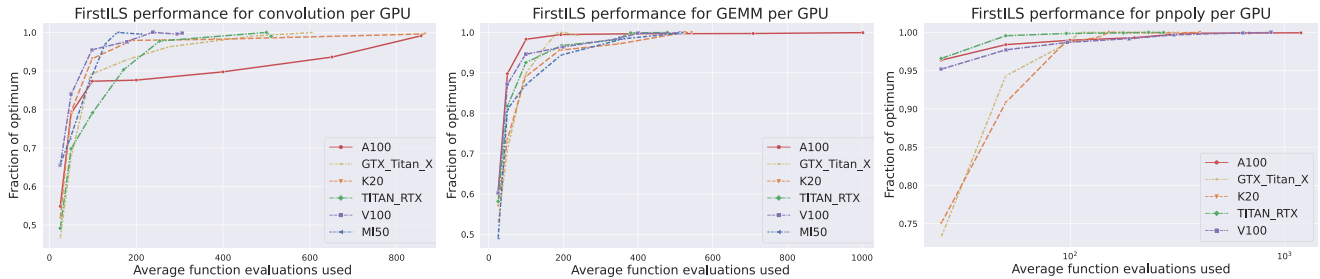
Fig. 5. FirstILS : Fraction of optimal runtime for different budgets (per GPU). Each point is the average fraction of optimal runtime found (y-axis) for each budget, with respect to the average number of evaluations actually used (x-axis) for that budget. Function evaluations used counts only the unique settings that were visited. Left: convolution kernel. Middle: GEMM kernel. Right: PnPoly kernel (logarithmic x-axis).
