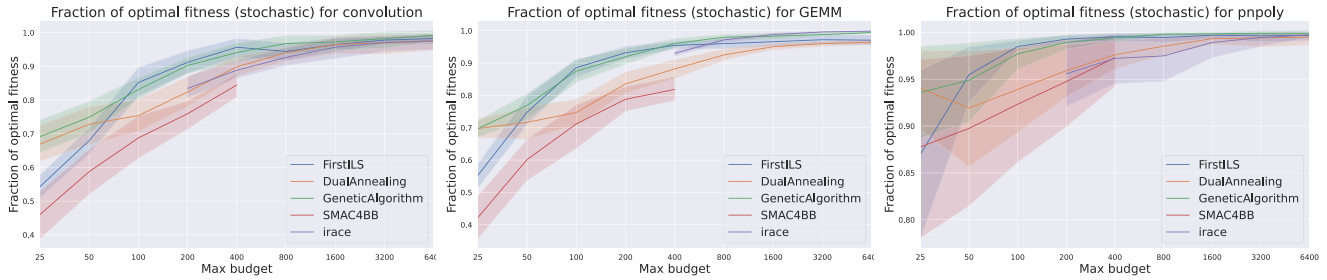
Fig. 2. Fraction of optimal runtime for max budget supplied over all GPUs. Each point is the mean fraction of optimal runtime found (y-axis) for each budget limit (x-axis) over all GPUs, with the shaded region indicating 95% confidence interval. Left: convolution kernel. Middle: GEMM kernel. Right: PnPoly kernel (logarithmic x-axis).
