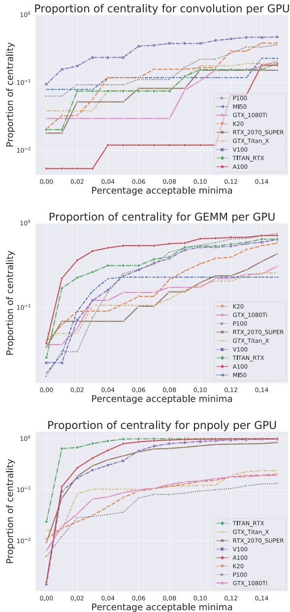
Fig. 7. Proportion of centrality for FFGs for each GPU. The proportion of centrality is computed by taking the sum of PageRank centrality for local minima within p\% of the optimal fitness, divided by the total PageRank centrality of all local minima. From top to bottom are convolution, GEMM, and PnPoly kernel.
