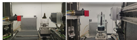
Fig. 4 Scanning setup for the case study objects in the Flex-ray scanner
