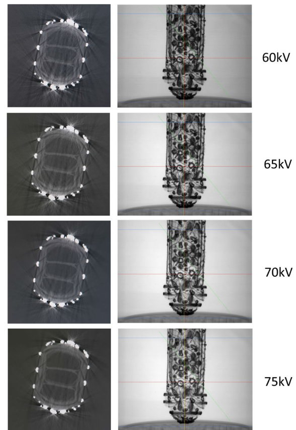
Fig. 10 From top to bottom: Reconstruction slices and radiographs of the “Purple velvet knife holder” of scans 2–5 with the specific acquisition parameters listed in Table 2. The cross-section images shown are taken from slice 1084
