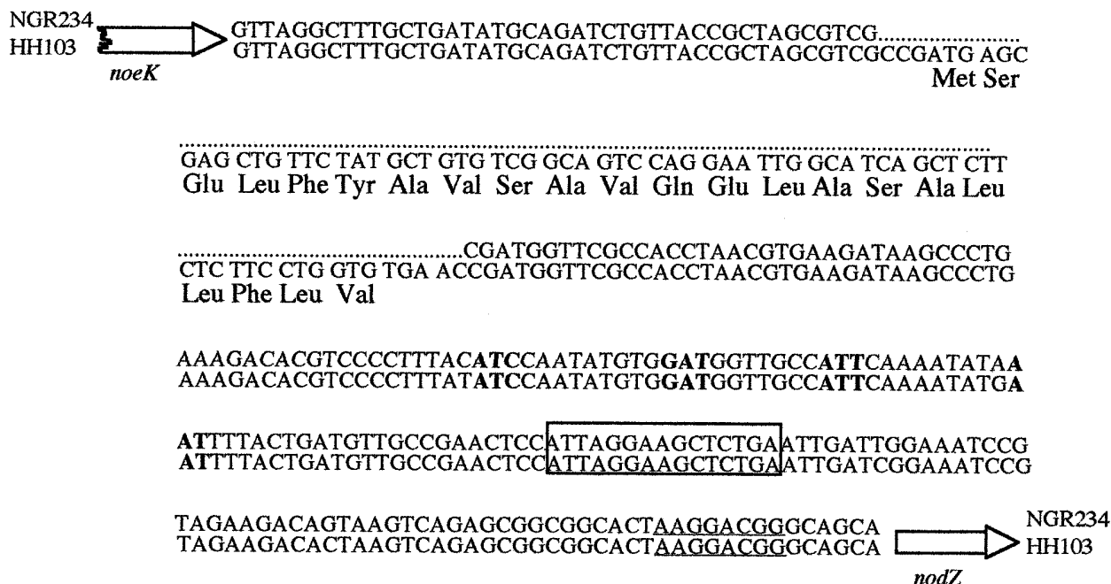
Fig. 4. Nucleotide and deduced amino acid sequences deduced of the nifW -like open reading frame (ORF) that lies within the noeK - nodZ intergenic region. The putative NodR-binding site is boxed; the putative ribosome-binding site of nodZ is underlined. The characteristic ATC, GAT, ATT, and AAT nucleotide blocks within the nod box (Goethals et al. 1992) are in boldface.
