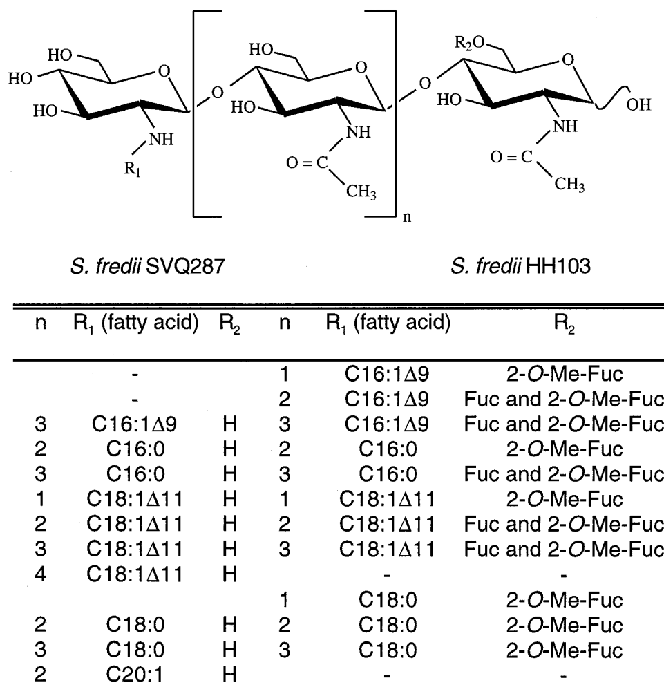
Fig. 2. Summary of the lipochitooligosaccharide (LCO) structures produced by mutant derivative SVQ287 compared with those from strain HH103 (Gil-Serrano et al. 1997).
