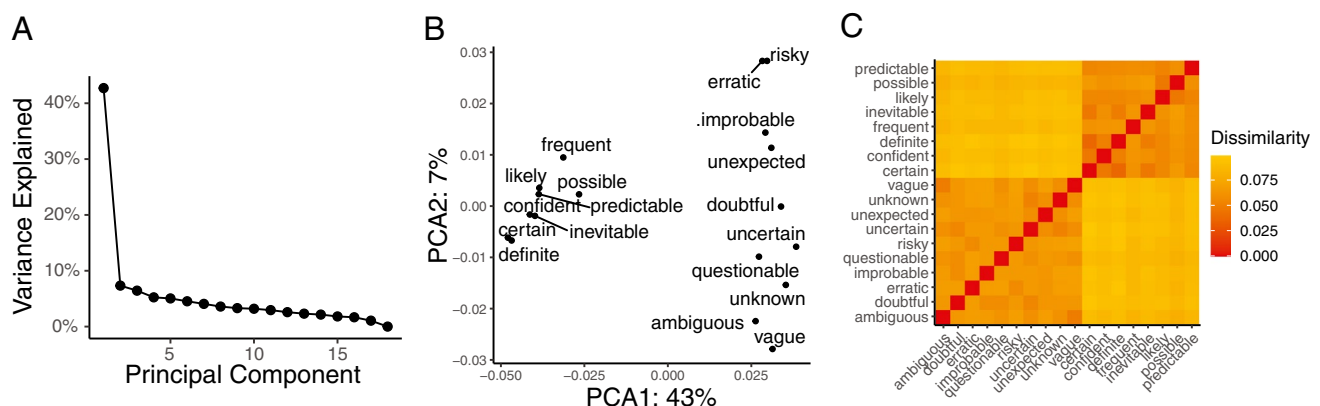
Fig. 3 Conceptual representations of uncertainty are one dimensional and organized by valence or probability. A. The percentage of variance explained for principal dimension from the similarity data reveals a sharp kink after the first component, illustrating that the
