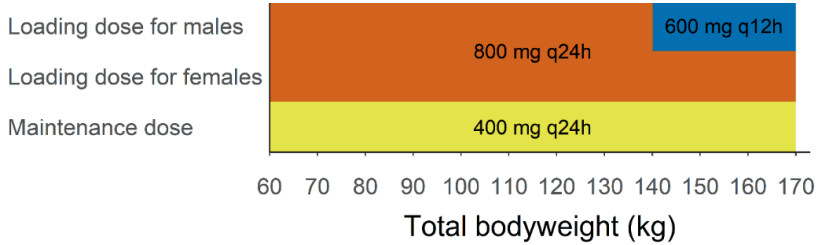
Figure 5. Model-derived IV loading and maintenance dose recommendations for fluconazole for achieving a target AUC_{24\text{ h}} > 200\text{ mg}\cdot\text{h/L} for the first day of treatment in female and male subjects of various TBWs.
