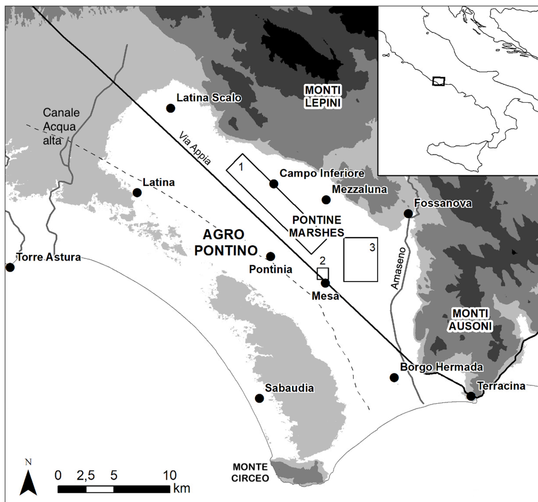
Figure 1. The Agro Pontino with topographic names of major locations and landforms. Areas studied in detail: (1) Fiume Murillo area; (2) Mesa area; (3) La Cotarda area. - - - = Southwestern border of Pontine Marshes.
